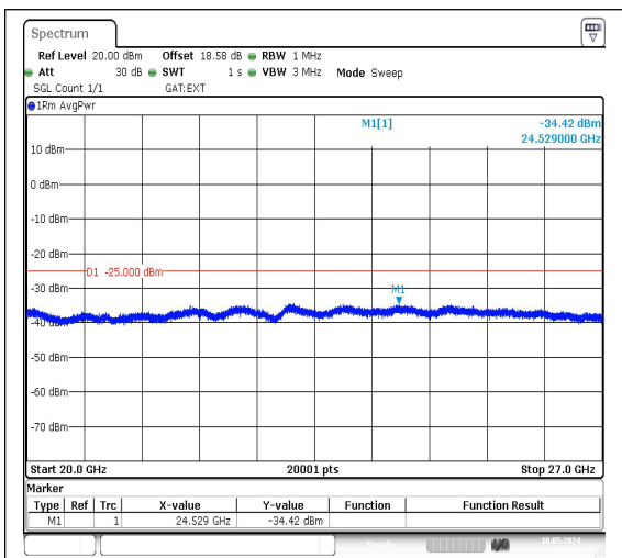
Band38_15MHz_QPSK_38175_1RB#0_20000~27000_20000~27000
