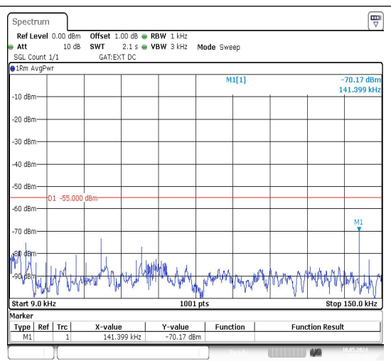
Band38_10MHz_16QAM_37800_1RB#0_0.009~0.15
