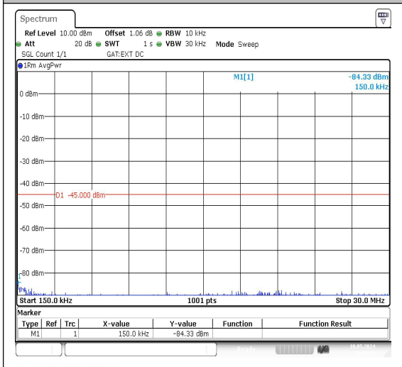
Band38_10MHz_16QAM_38200_1RB#0_0.15~30_0.15~30
