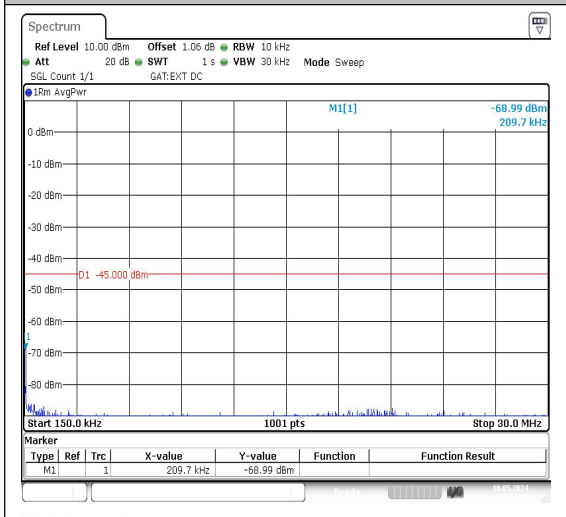
Band38_10MHz_16QAM_37800_1RB#0_0.15~30
