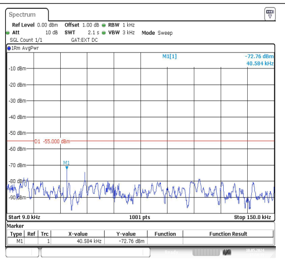
Band38_10MHz_16QAM_38000_1RB#0_0.009~0.15
