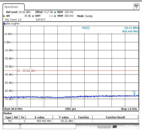
Band38_10MHz_16QAM_38200_1RB#0_30~1000_30~1000
