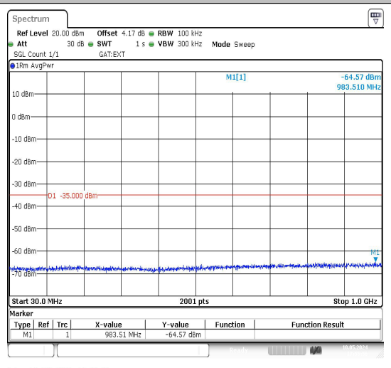
Band38_10MHz_16QAM_37800_1RB#0_30~1000
