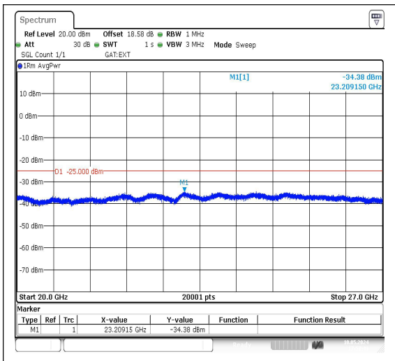
Band38_10MHz_QPSK_38000_1RB#0_20000~27000
