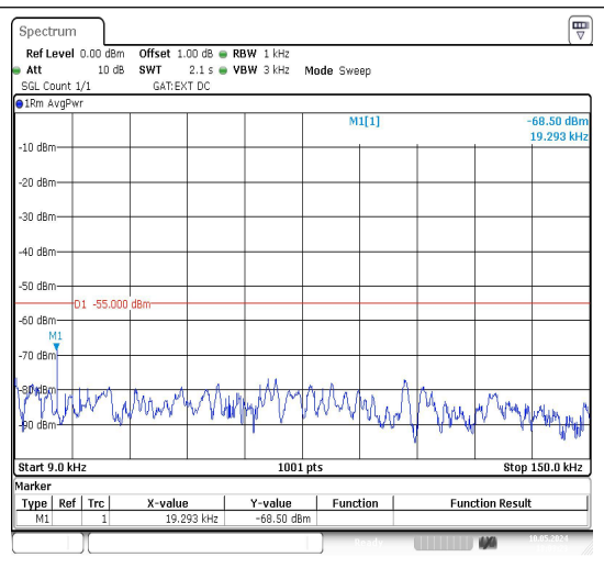
Band38_10MHz_16QAM_38200_1RB#0_0.009~0.15_0.009~0.15
