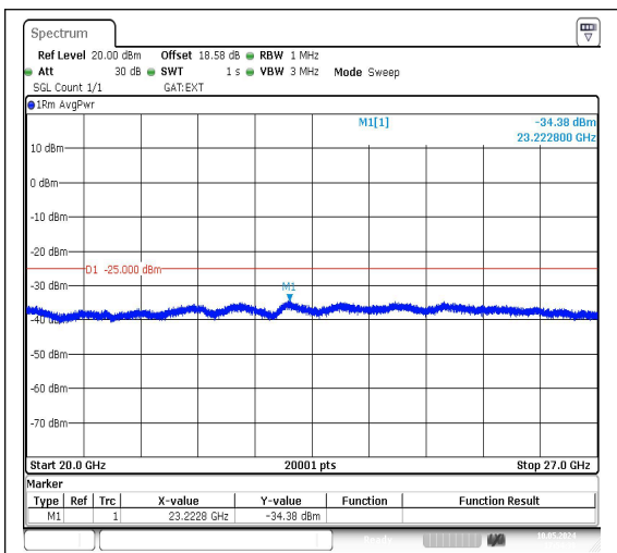
Band38_10MHz_QPSK_37800_1RB#0_20000~27000
