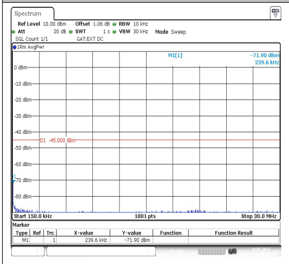
Band38_5MHz_16QAM_38000_1RB#0_0.15~30_0.15~30
