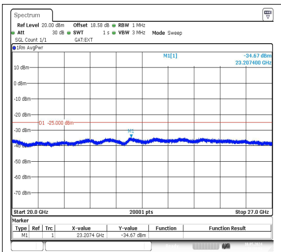
Band38_5MHz_QPSK_38225_1RB#0_20000~27000
