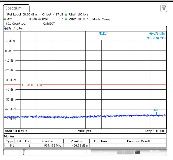
Band38_5MHz_16QAM_38000_1RB#0_30~1000_30~1000
