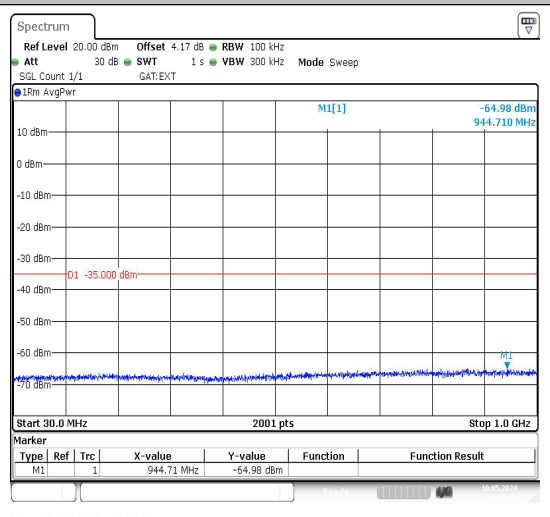
Band38_5MHz_16QAM_38225_1RB#0_30~1000
