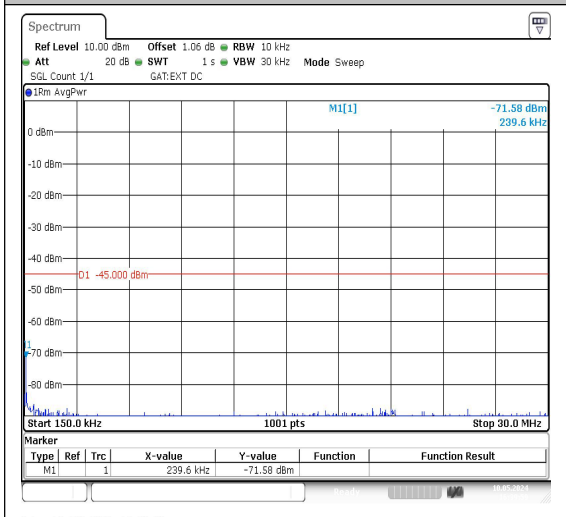
Band38_5MHz_16QAM_38225_1RB#0_0.15~30
