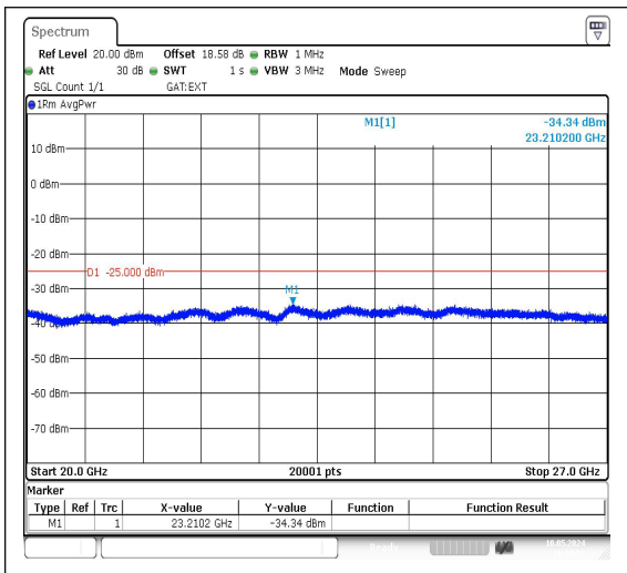
Band38_5MHz_QPSK_38000_1RB#0_20000~27000_000_20000~27000
