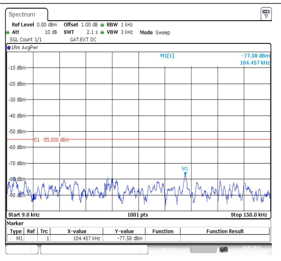
Band38_5MHz_16QAM_38000_1RB#0_0.009~0.1_5_0.009~0.15
