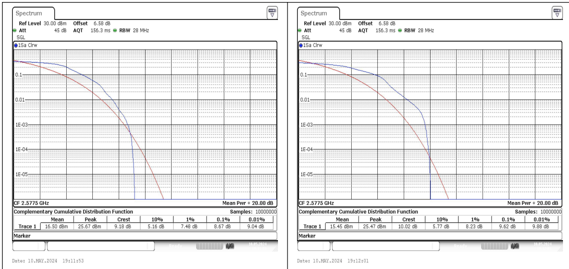
Band38-15MHz-QPSK-37825-1RB#0-PASS Band38-15MHz-16QAM-37825-1RB#0-PASS
