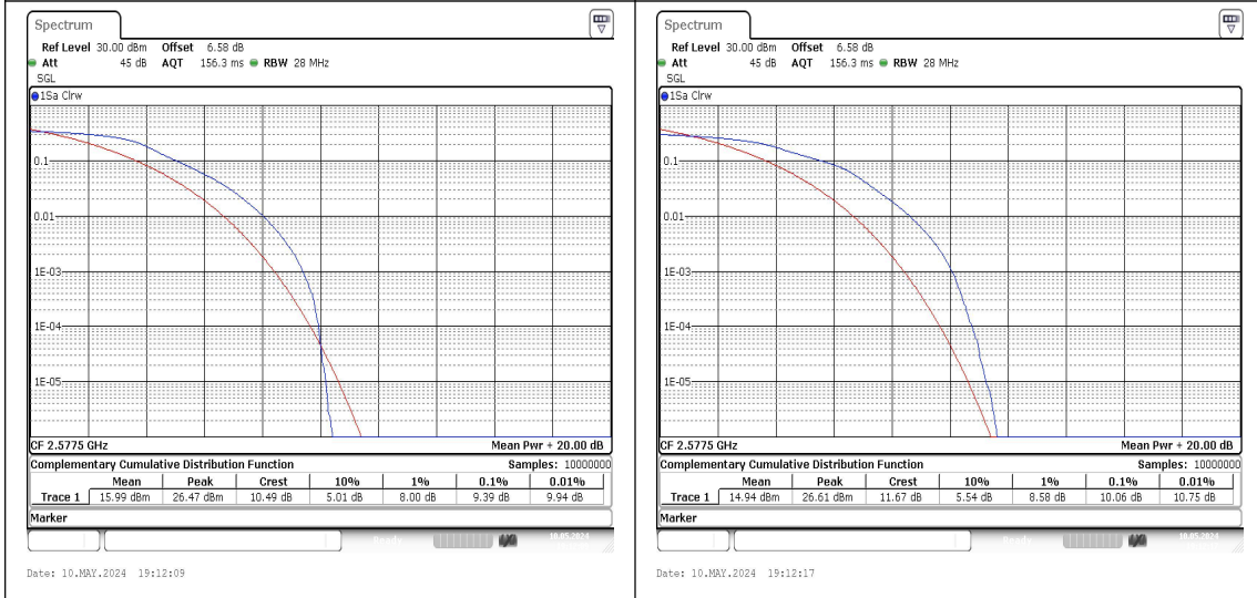
Band38-15MHz-QPSK-37825-75RB#0-PASS Band38-15MHz-16QAM-37825-75RB#0-PASS
