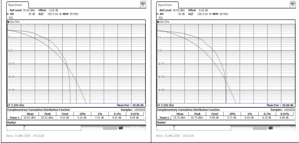
Band38-15MHz-QPSK-38000-1RB#0-PASS Band38-15MHz-16QAM-38000-1RB#0-PASS
