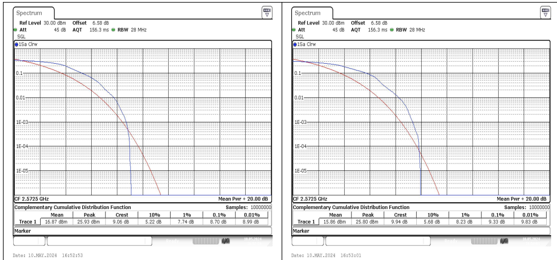
Band38-5MHz-QPSK-37775-1RB#0-PASS
