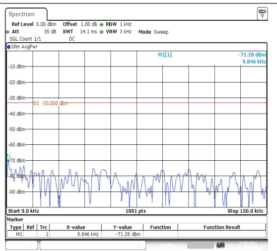
Band26_10MHz_16QAM_26915_1RB#0_0.009~0.15
