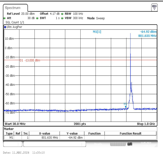
Band26_10MHz_16QAM_26915_1RB#0_30~1000
