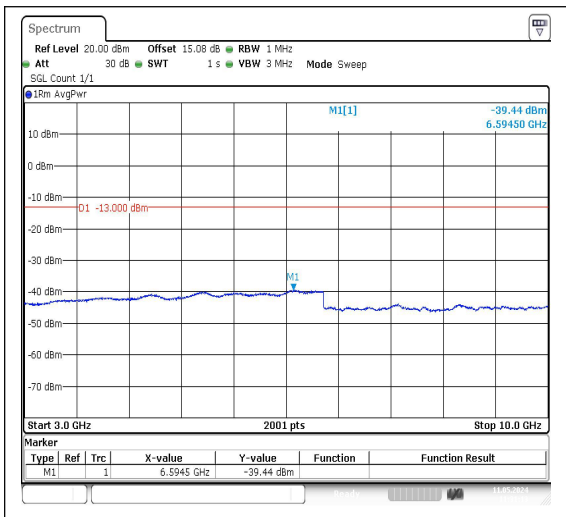
Band26_10MHz_QPSK_26990_1RB#0_3000~10000_3000~10000
