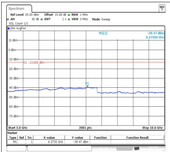
Band26_10MHz_QPSK_26915_1RB#0_3000~10000
