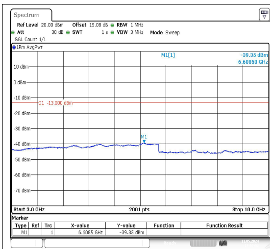
Band26_15MHz_QPSK_26865_1RB#0_3000~10000
