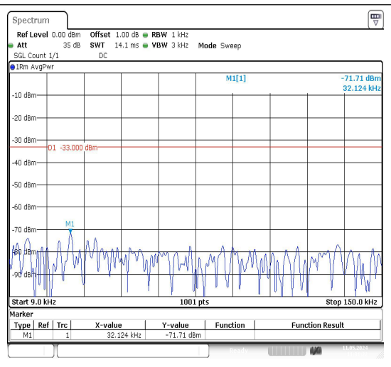
Band26_10MHz_16QAM_26990_1RB#0_0.009~0.15_0.009~0.15
