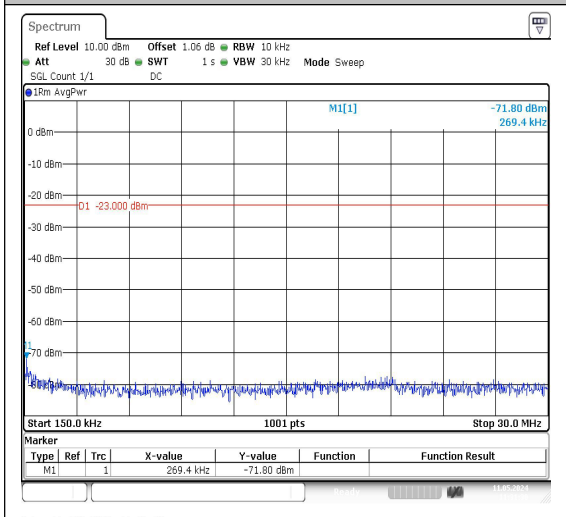
Band26_10MHz_QPSK_26990_1RB#0_0.15~30_0.15~30
