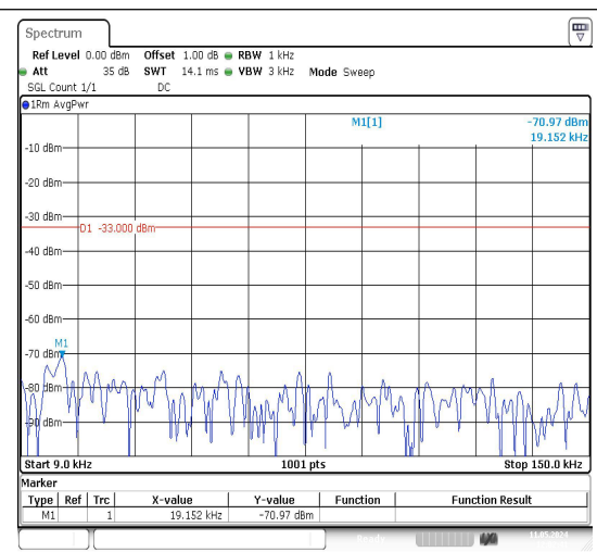
Band26_15MHz_16QAM_26865_1RB#0_0.009~0.15
