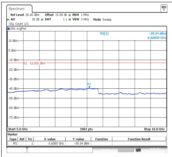
Band26_5MHz_QPSK_27015_1RB#0_3000~10000
