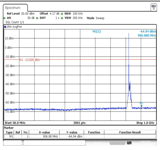
Band26_10MHz_16QAM_26840_1RB#0_30~1000
