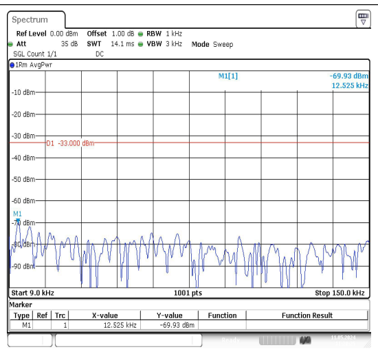
Band26_10MHz_16QAM_26840_1RB#0_0.009~0.15
