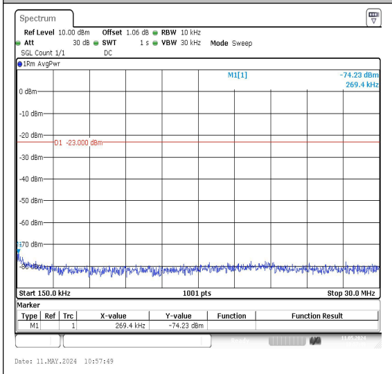
Band26_5MHz_16QAM_27015_1RB#0_0.15~30
