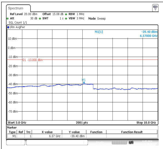
Band26_10MHz_QPSK_26840_1RB#0_3000~10000
