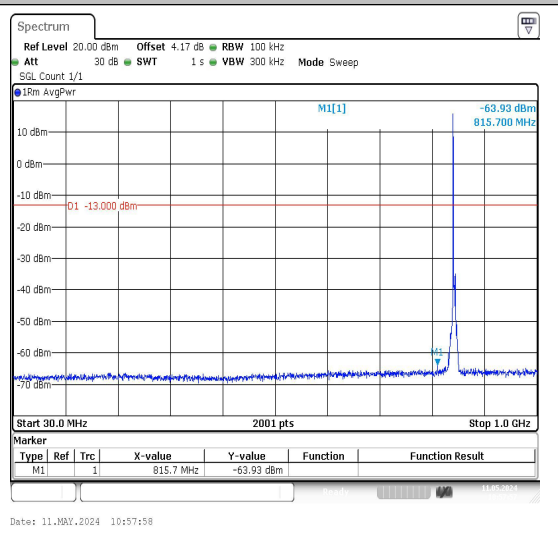
Band26_5MHz_16QAM_27015_1RB#0_30~1000
