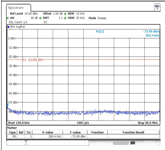
Band26_10MHz_16QAM_26840_1RB#0_0.15~30
