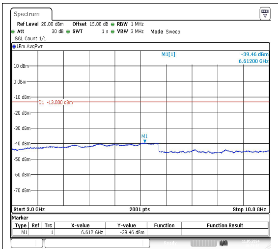
Band26_3MHz_QPSK_27025_1RB#0_3000~10000
