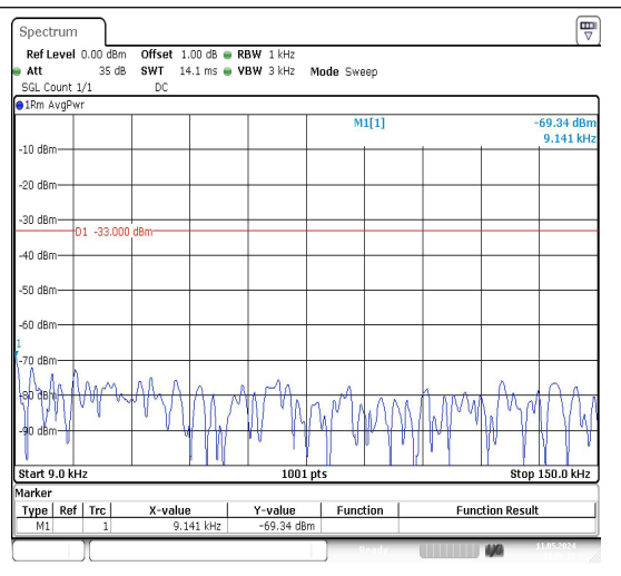
Band26_5MHz_16QAM_26915_1RB#0_0.009~0.15
