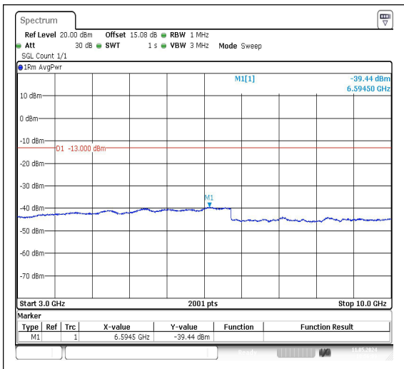
Band26_5MHz_QPSK_26915_1RB#0_3000~10000
