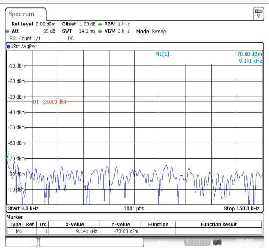
Band26_3MHz_16QAM_27025_1RB#0_0.009~0.15
