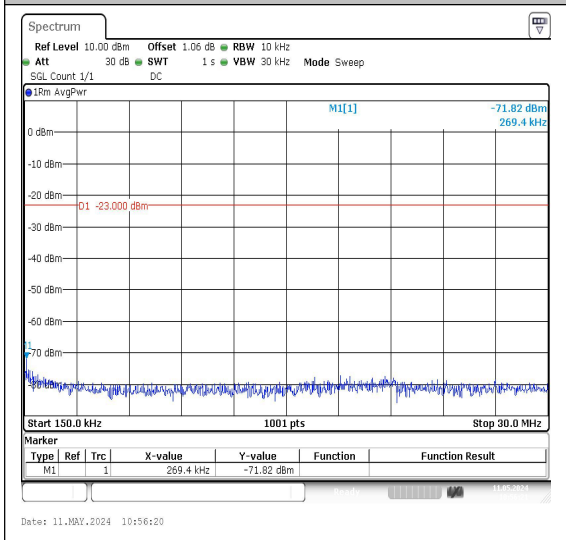
Band26_5MHz_16QAM_26915_1RB#0_0.15~30
