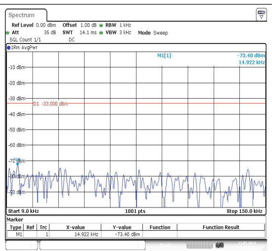
Band26_1.4MHz_16QAM_27033_1RB#0_0.009~0.15_0.009~0.15
