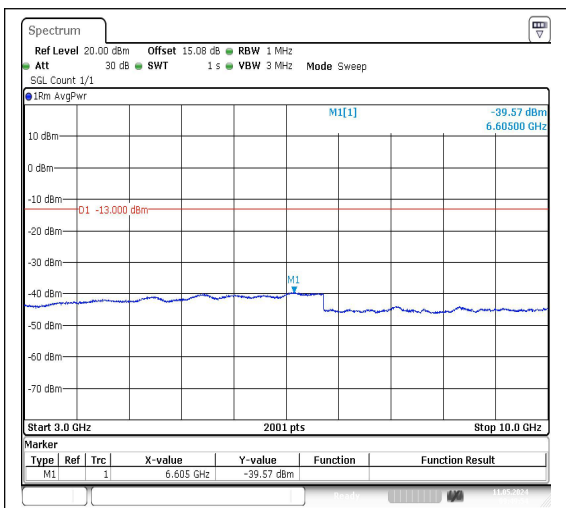
Band26_1.4MHz_QPSK_27033_1RB#0_3000~1000_3000~10000
