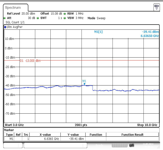
Band26_1.4MHz_16QAM_26915_1RB#0_30~100_0_30~100
