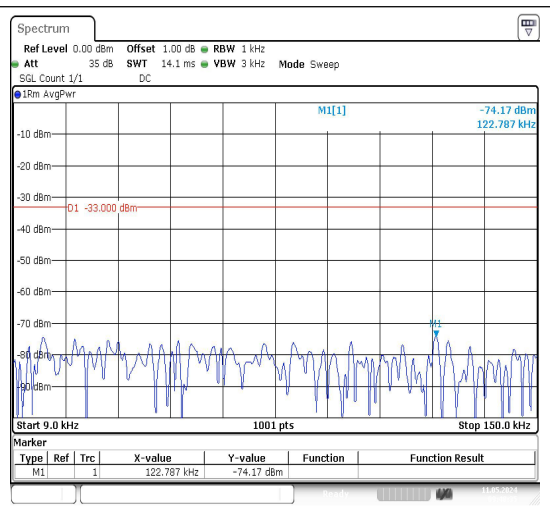
Band26_1.4MHz_16QAM_26915_1RB#0_0.009~0.15_0.009~0.15
