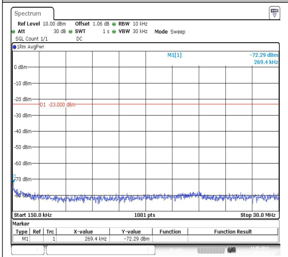
Band26_1.4MHz_QPSK_26915_1RB#0_3000~1000_3000~10000
