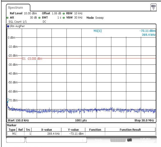
Band26_1.4MHz_16QAM_27033_1RB#0_0.15~30_0.15~30
