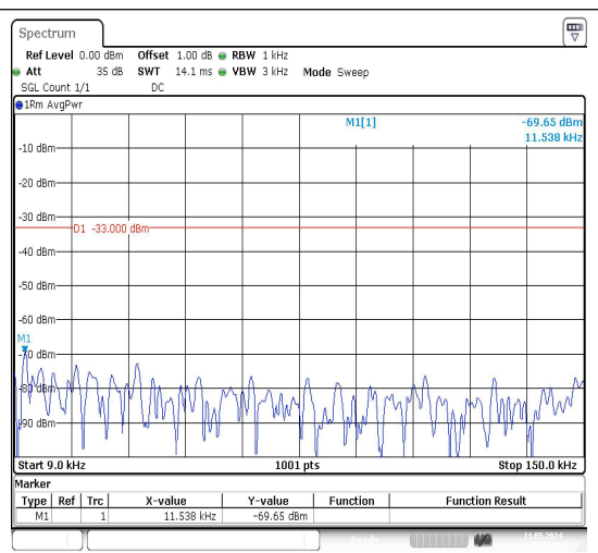
Band26_1.4MHz_16QAM_26797_1RB#0_0.009~0.15_0.009~0.15
