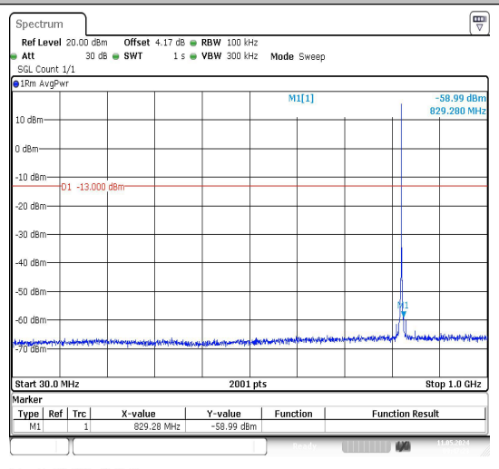
Band26_1.4MHz_16QAM_26797_1RB#0_30~100_0_30~1000
