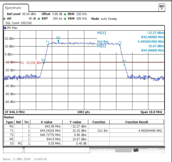
26(824-849)-5MHz-16QAM-27015-25RB#0-PASS
