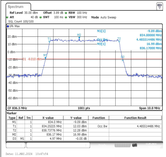
26(824-849)-5MHz-QPSK-26915-25RB#0-PASS
