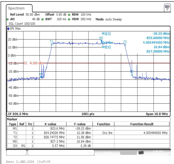
26(824-849)-5MHz-QPSK-26815-25RB#0-PASS
