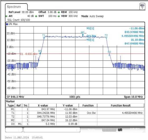
26(824-849)-5MHz-QPSK-27015-25RB#0-PASS
