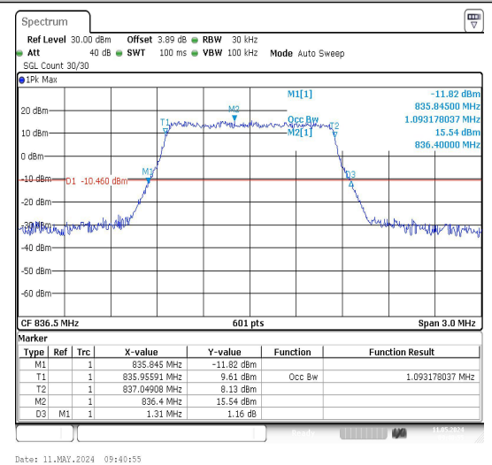
26(824-849)-1.4MHz-16QAM-26915-6RB#0-PASS
