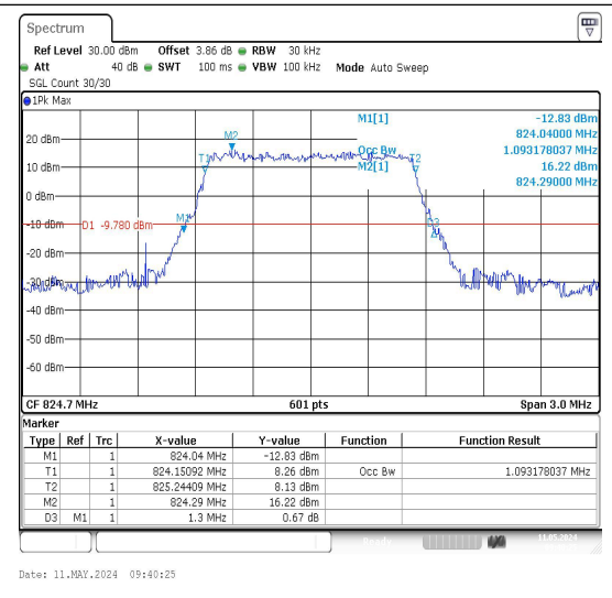
26(824-849)-1.4MHz-16QAM-26797-6RB#0-PASS
