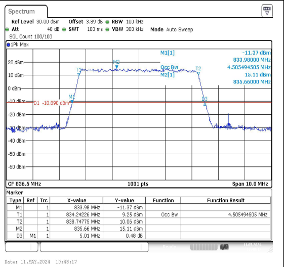
26(824-849)-5MHz-16QAM-26915-25RB#0-PASS
