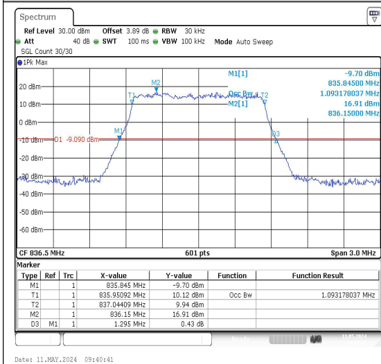
26(824-849)-1.4MHz-QPSK-26915-6RB#0-PASS
