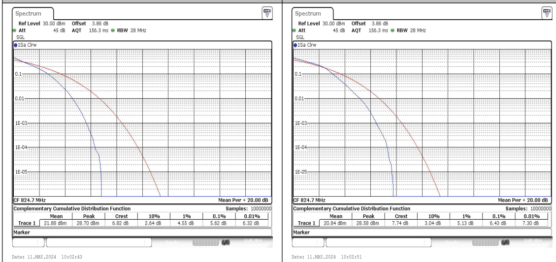
26(824-849)-1.4MHz-QPSK-26797-6RB#0-PASS 26(824-849)-1.4MHz-16QAM-26797-6RB#0-PASS
