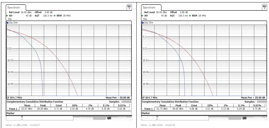
26(824-849)-1.4MHz-QPSK-26797-1RB#0-PASS 26(824-849)-1.4MHz-16QAM-26797-1RB#0-PASS
