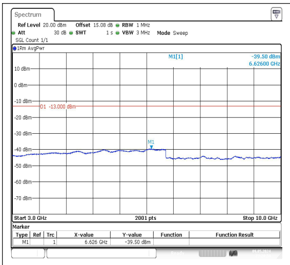
Band26_5MHz_QPSK_26740_1RB#0_3000~10000
