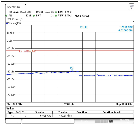
Band26_5MHz_QPSK_26765_1RB#0_3000~10000
