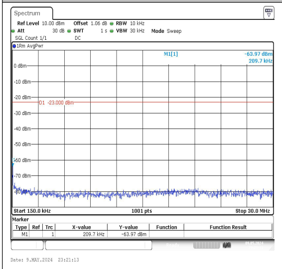
Band26_5MHz_16QAM_26740_1RB#0_0.15~30
