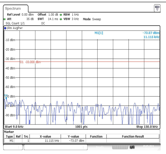
Band26_5MHz_16QAM_26740_1RB#0_0.009~0.15
