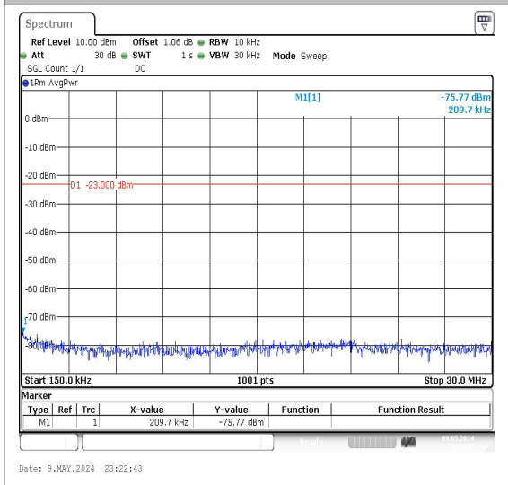
Band26_5MHz_16QAM_26765_1RB#0_0.15~30
