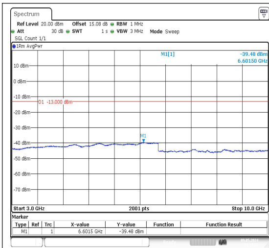
Band26_5MHz_QPSK_26715_1RB#0_3000~10000
