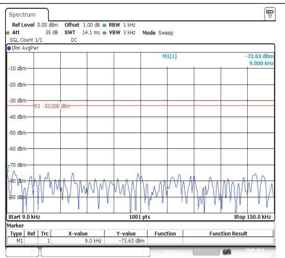
Band26_5MHz_16QAM_26765_1RB#0_0.009~0.15
