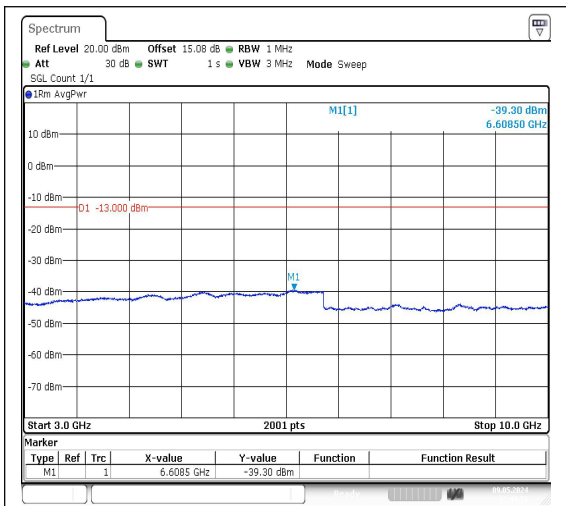
Band26_3MHz_QPSK_26740_1RB#0_3000~10000_00_3000~10000
