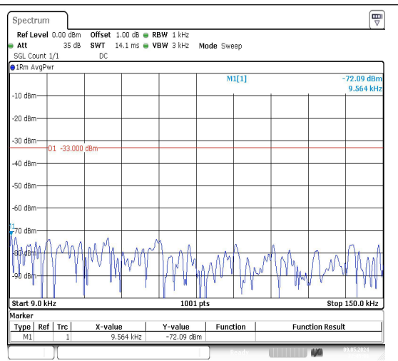
Band26_3MHz_16QAM_26740_1RB#0_0.009~0.15_5_0.009~0.15
