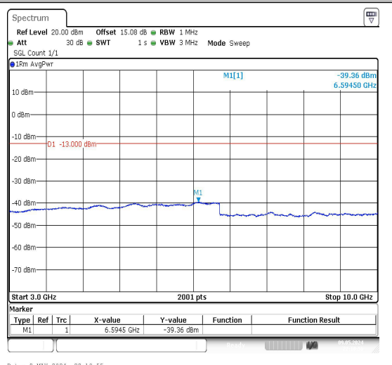
Band26_1.4MHz_16QAM_26740_1RB#0_30~100_0_30~100
