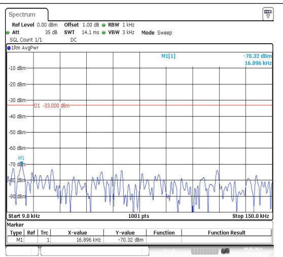
Band26_1.4MHz_16QAM_26783_1RB#0_0.009~0.15
