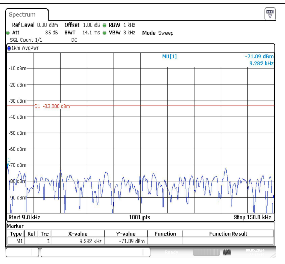
Band26_1.4MHz_16QAM_26740_1RB#0_0.009~0.15_0.009~0.15
