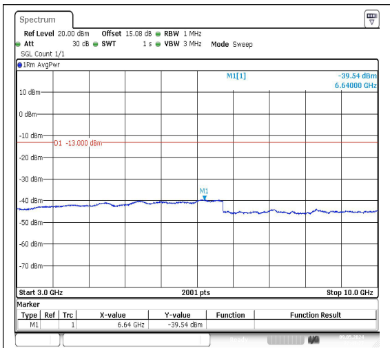
Band26_3MHz_QPSK_26705_1RB#0_3000~10000
