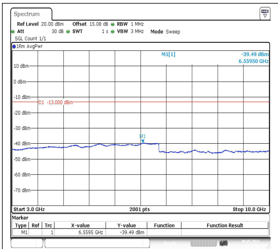
Band26_1.4MHz_QPSK_26783_1RB#0_3000~10000
