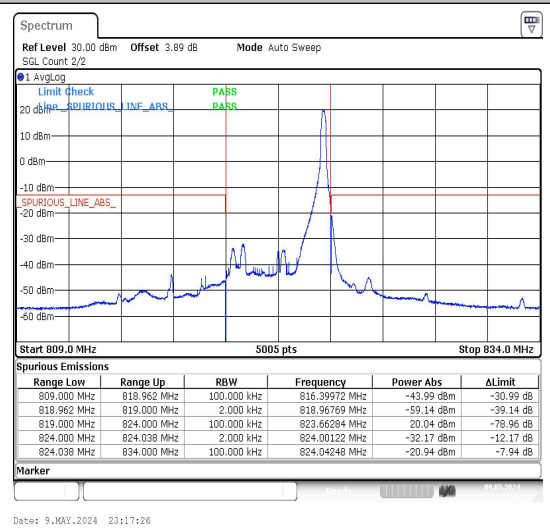
Band26_5MHz_16QAM_26765_1RB#24
