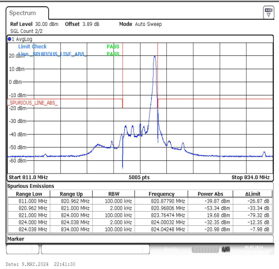
Band26_3MHz_16QAM_26775_1RB#14
