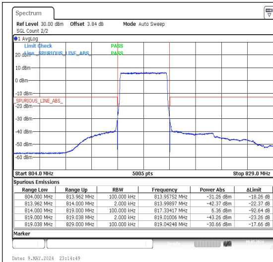
Band26_5MHz_QPSK_26715_25RB#0
