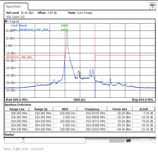
Band26_5MHz_16QAM_26765_1RB#0
