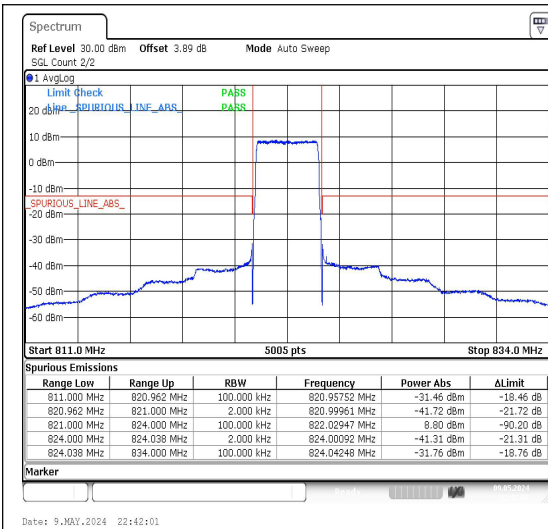
Band26_3MHz_QPSK_26775_15RB#0
