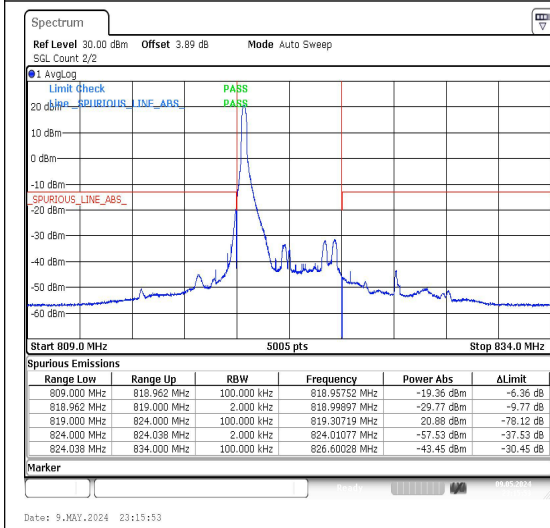
Band26_5MHz_QPSK_26765_1RB#0
