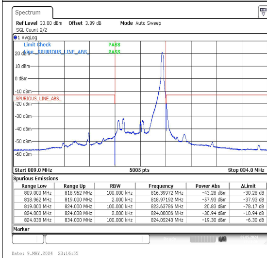
Band26_5MHz_QPSK_26765_1RB#24
