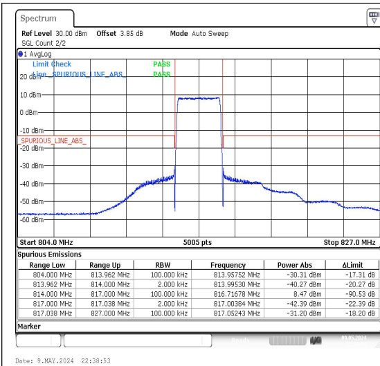
Band26_3MHz_QPSK_26705_15RB#0
