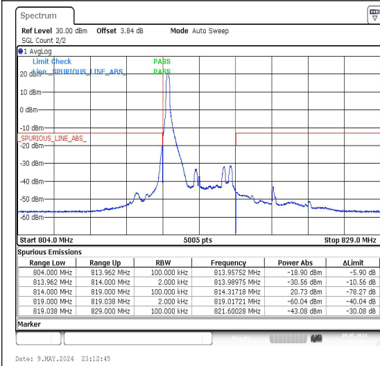
Band26_5MHz_QPSK_26715_1RB#0
