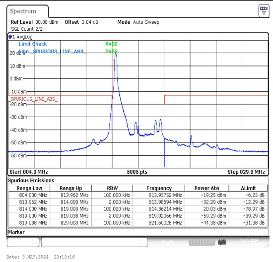
Band26_5MHz_16QAM_26715_1RB#0
