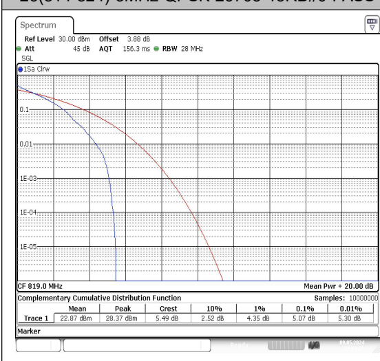
26(814-824)-3MHz-QPSK-26740-1RB#0-PASS
