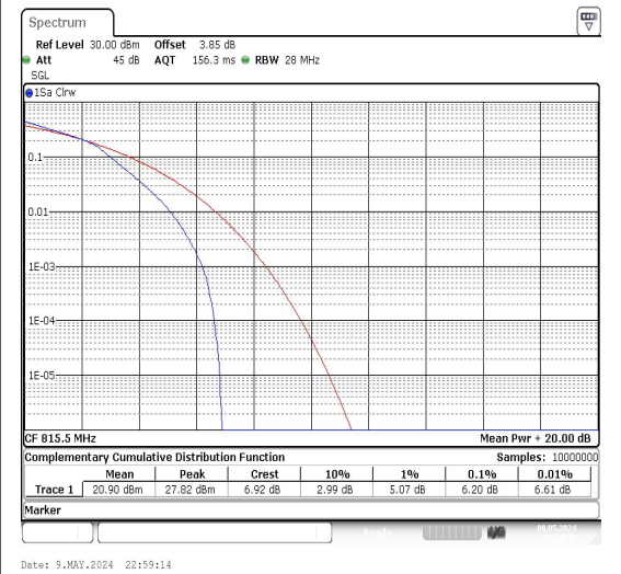
26(814-824)-3MHz-16QAM-26705-15RB#0-PASS
