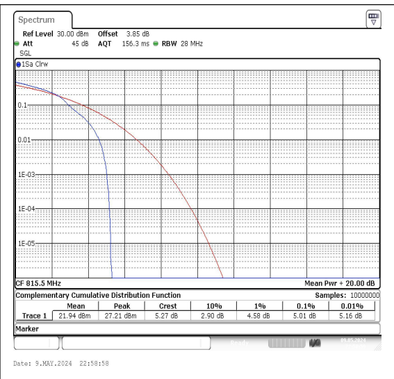
26(814-824)-3MHz-16QAM-26705-1RB#0-PASS
