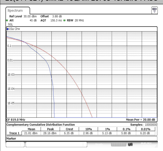
26(814-824)-3MHz-16QAM-26740-1RB#0-PASS
