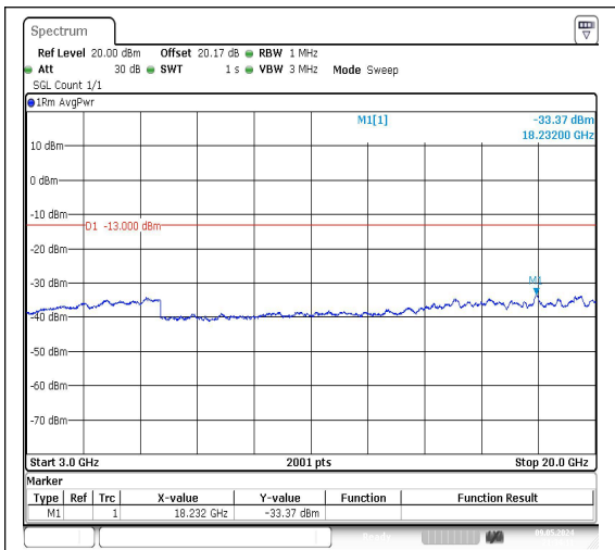
Band25_20MHz_QPSK_26365_1RB#0_3000~2000_3000~20000
