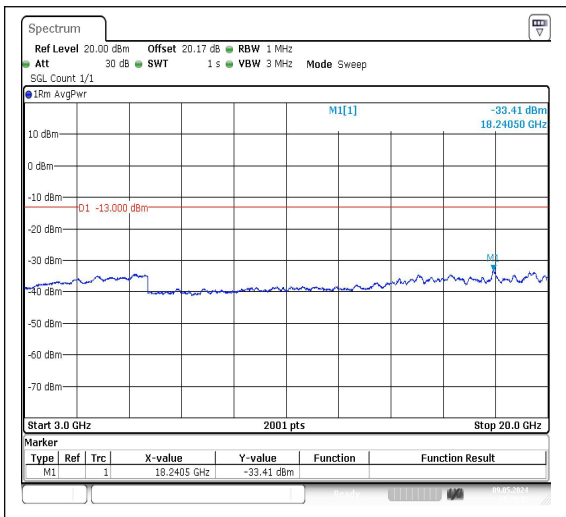
Band25_10MHz_QPSK_26365_1RB#0_3000~2000_3000~20000
