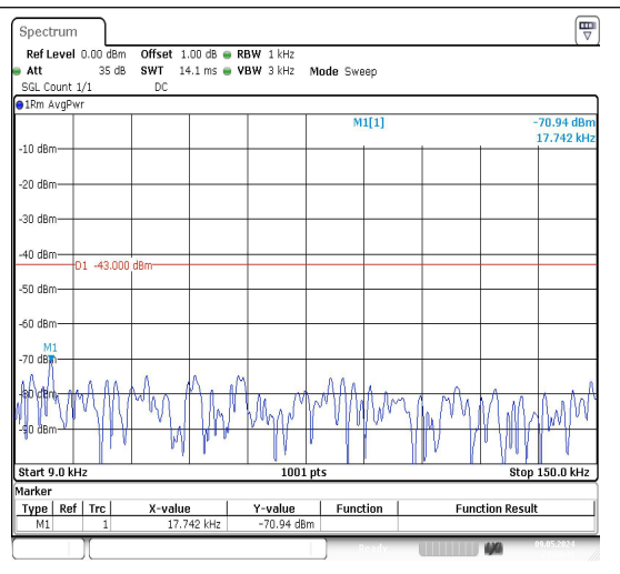
Band25_10MHz_16QAM_26365_1RB#0_0.009~0.15_0.009~0.15
