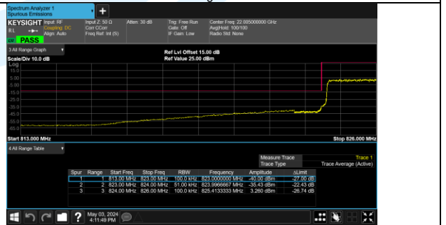
Band 5 20425/826.5/Low 64QAM 25@0
