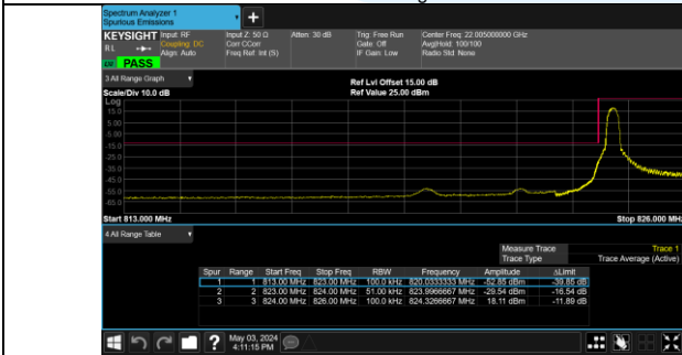
Band 5 20425/826.5/Low 64QAM 1@0
