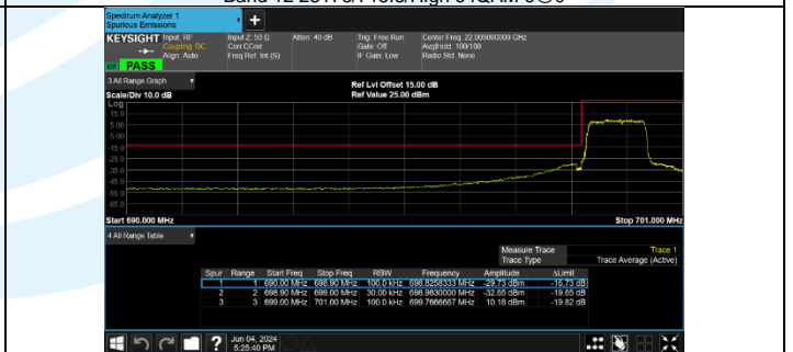
Band 12 23017/699.7/Low 64QAM 6@0
