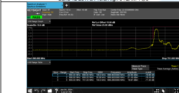
Band 12 23017/699.7/Low 64QAM 1@0
