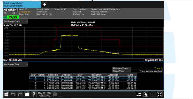
Band 13 23205/779.5/Low 64QAM 25@0
