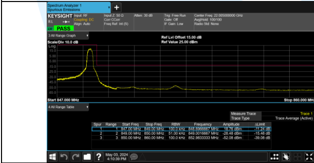
Band 5 20625/846.5/High 64QAM 1@24
