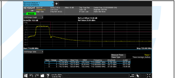
Band 12 23173/715.3/High 64QAM 6@0
