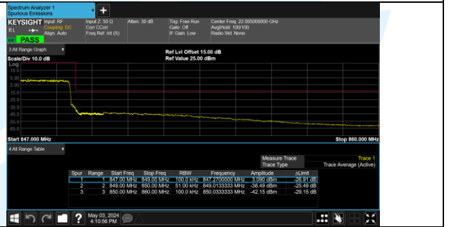
Band 5 20625/846.5/High 64QAM 25@0
