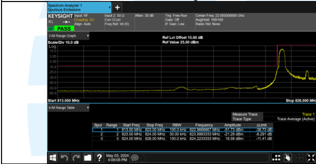
Band 5 20415/825.5/Low 64QAM 1@0
