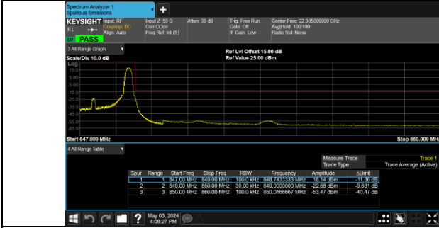
Band 5 20635/847.5/High 64QAM 1@14
