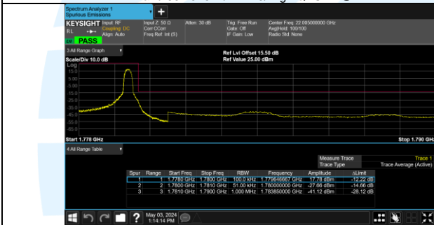
Band 66 132647/1777.5/High 16QAM 1@24
