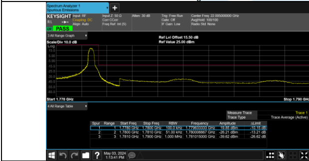
Band 66 132647/1777.5/High QPSK 1@24
