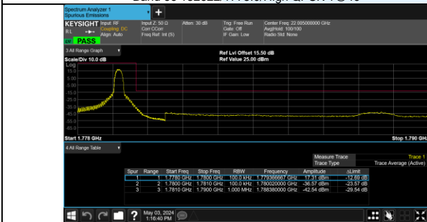
Band 66 132622/1775.0/High 16QAM 1@49
