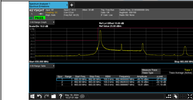
Band 71 133172/668.0/Low QPSK 1@0
