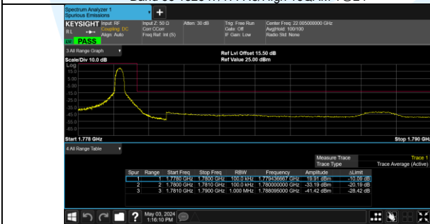
Band 66 132622/1775.0/High QPSK 1@49
