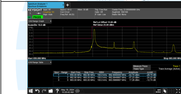
Band 71 133172/668.0/Low 16QAM 1@0
