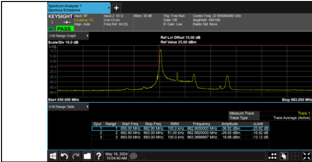
Band 71 133147/665.5/Low 16QAM 1@0
