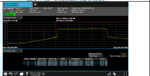
Band 71 133197/670.5/Low QPSK 75@0
