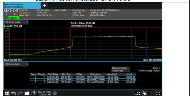
Band 71 133197/670.5/Low 16QAM 75@0
