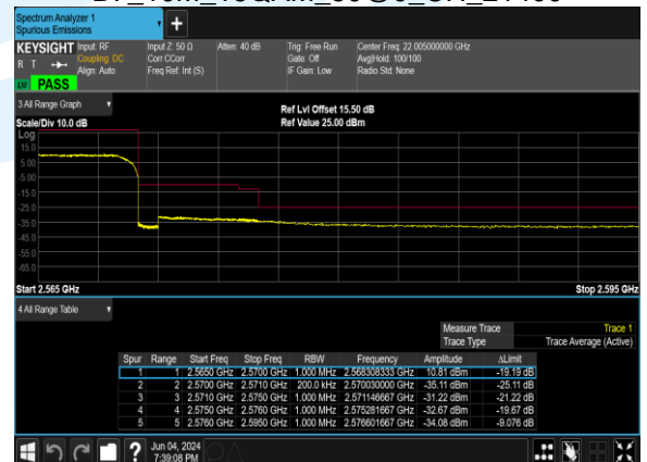
B7_10M_16QAM_50@0_CH_21400
