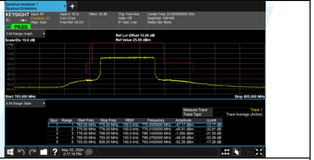
Band 13 23230/782.0/Low 16QAM 50@0
