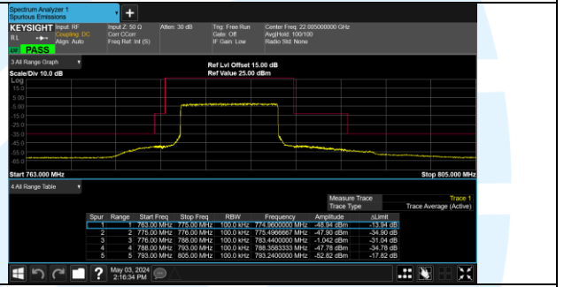
Band 13 23230/782.0/Low QPSK 50@0
