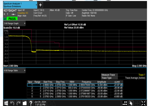
B7_15M_16QAM_75@0_CH_21375
