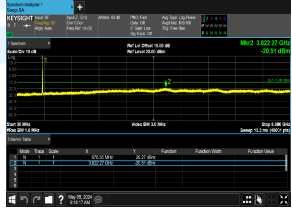
B71_10M_64QAM_1@0_CH_133297
