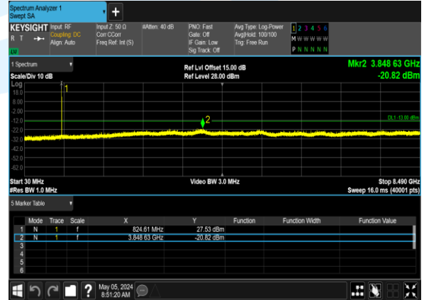
B5_5M_64QAM_1@0_CH_20425
