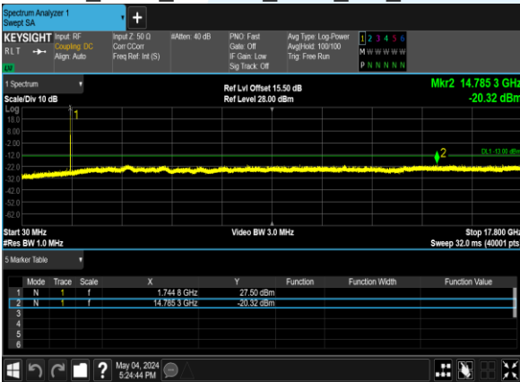
B66_1.4M_64QAM_1@0_CH_132322
