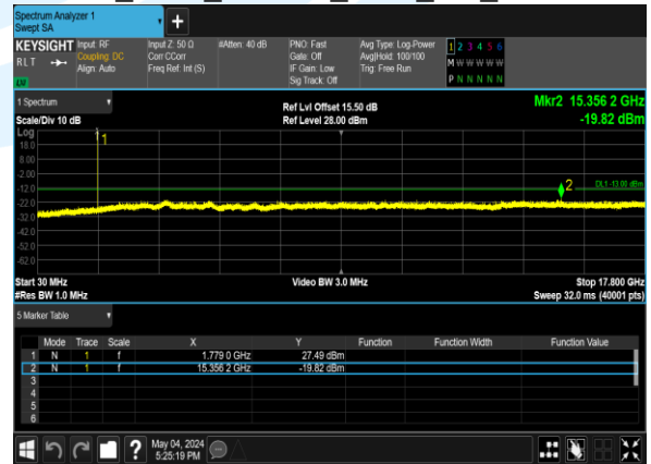
B66_1.4M_64QAM_1@0_CH_132665
