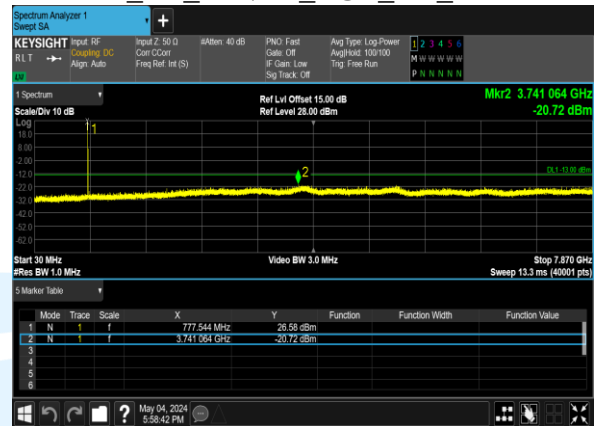
B13_5M_64QAM_1@0_CH_23205
