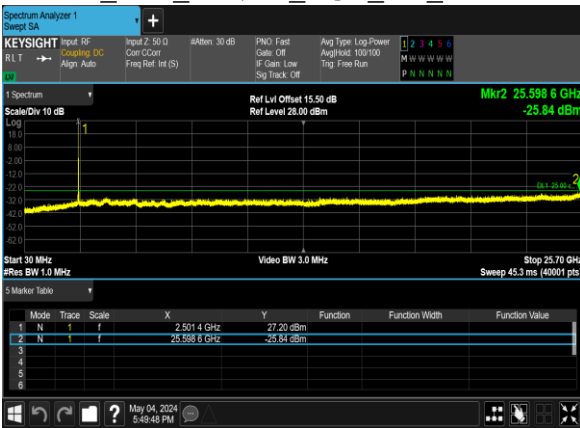
B7_20M_64QAM_1@0_CH_21350
