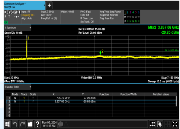
B17_5M_64QAM_1@0_CH_23755
