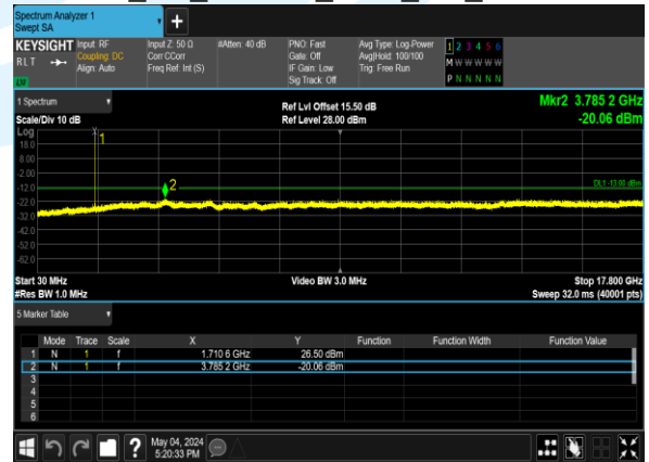
B66_5M_64QAM_1@0_CH_131997
