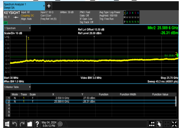
B7_10M_64QAM_1@0_CH_21100
