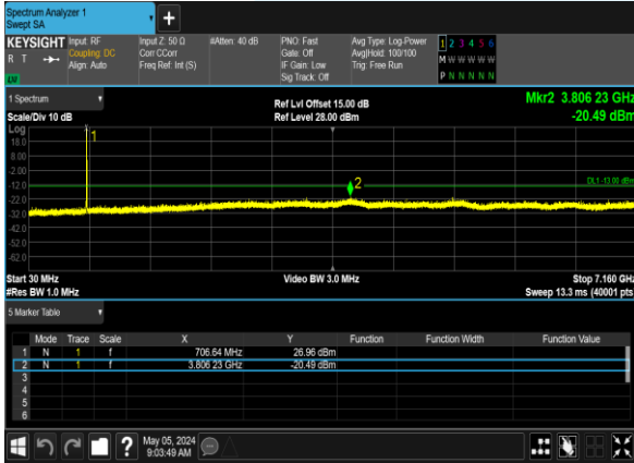
B12_10M_64QAM_1@0_CH_23130
