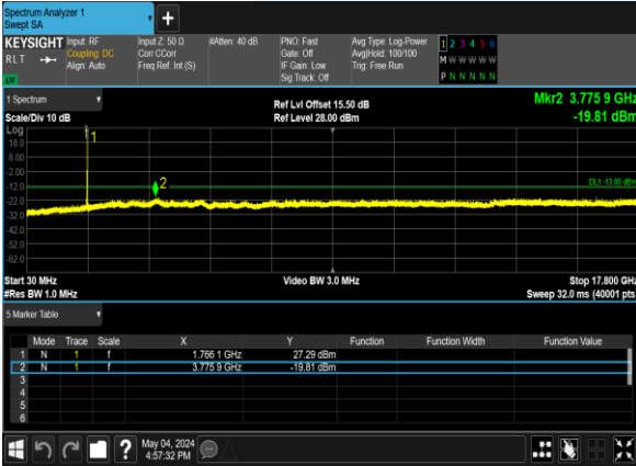
B66_15M_QPSK_1@0_CH_132597
