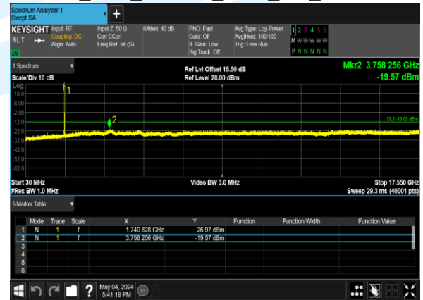
B4_15M_64QAM_1@0_CH_20325
