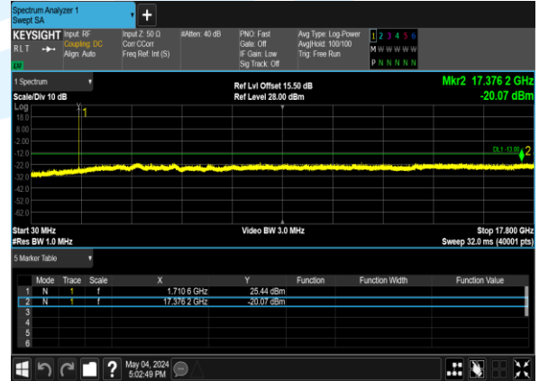
B66_5M_16QAM_1@0_CH_131997
