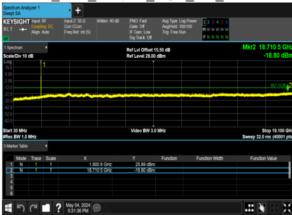
B2_5M_64QAM_1@0_CH_18900
