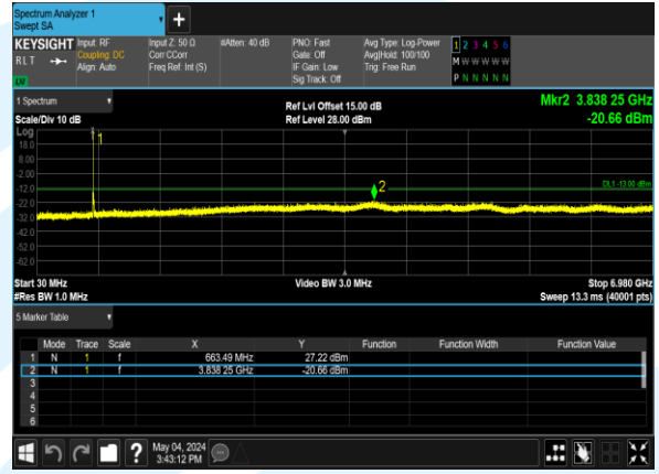
B71_5M_16QAM_1@0_CH_133297
