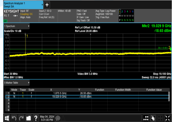
B2_10M_64QAM_1@0_CH_18900
