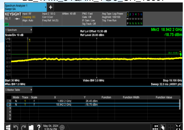
B2_1.4M_64QAM_1@0_CH_18607
