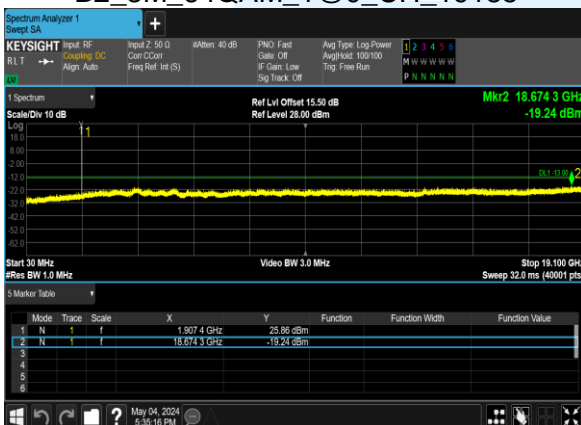
B2_3M_64QAM_1@0_CH_19185
