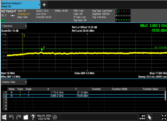
B66_5M_QPSK_1@0_CH_131997
