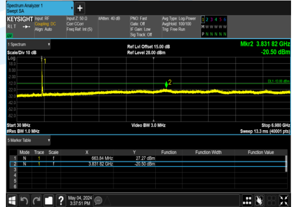
B71_15M_16QAM_1@0_CH_133197
