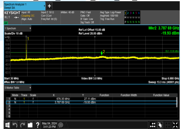
B71_10M_16QAM_1@0_CH_133297
