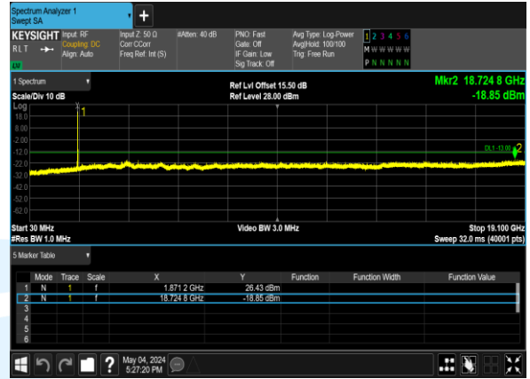
B2_15M_64QAM_1@0_CH_18675
