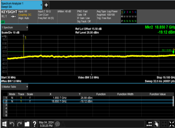
B2_10M_64QAM_1@0_CH_18650
