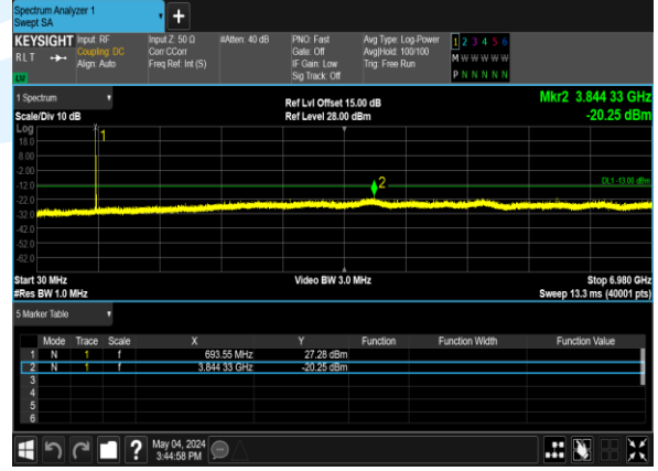
B71_5M_16QAM_1@0_CH_133447
