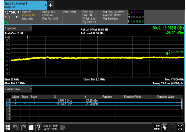
B66_15M_16QAM_1@0_CH_132597
