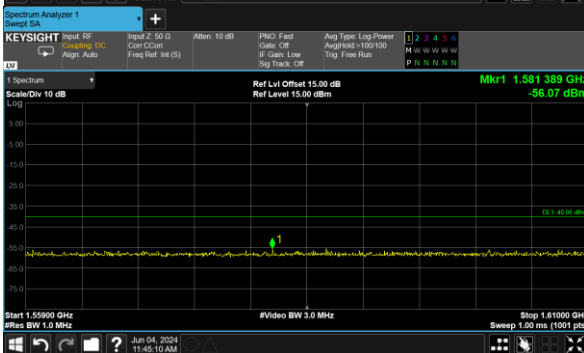
B13_5M_QPSK_1@0_CH_23255
