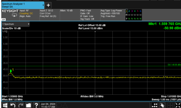
B13_5M_QPSK_1@0_CH_23205
