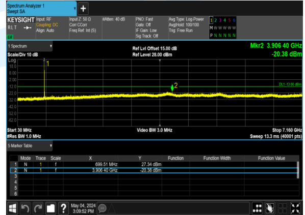
B12_5M_16QAM_1@0_CH_23035
