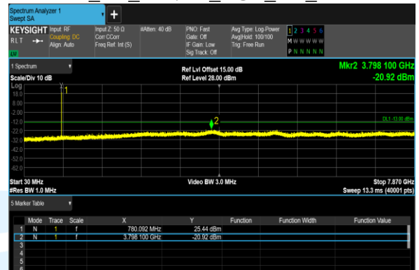
B13_5M_16QAM_1@0_CH_23230
