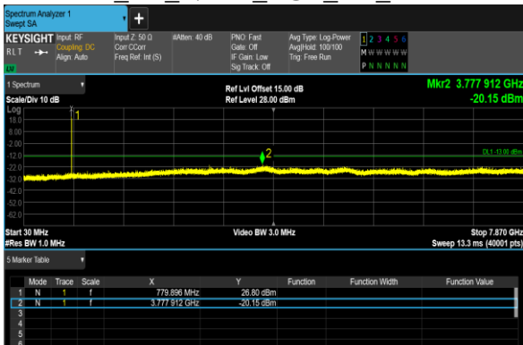
B13_5M_QPSK_1@0_CH_23230
