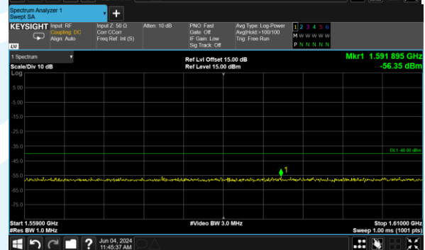
B13_5M_16QAM_1@0_CH_23255
