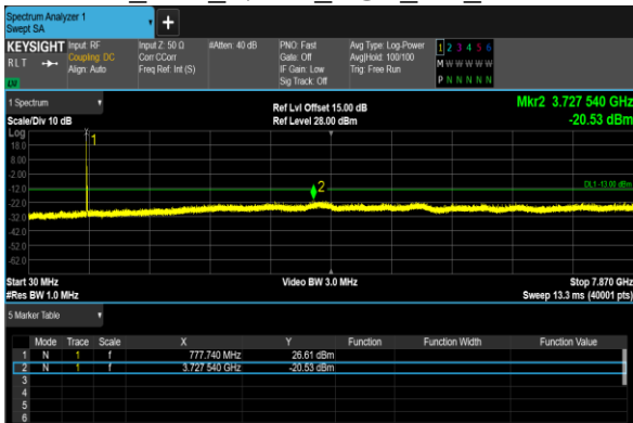
B13_10M_QPSK_1@0_CH_23230
