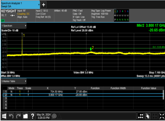
B17_5M_QPSK_1@0_CH_23755
