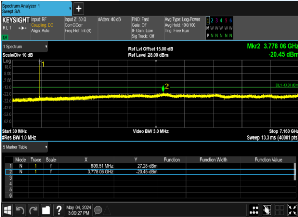
B12_5M_QPSK_1@0_CH_23035
