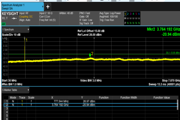
B13_5M_QPSK_1@0_CH_23205
