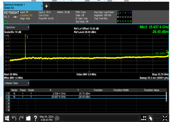
B7_20M_16QAM_1@0_CH_21350
