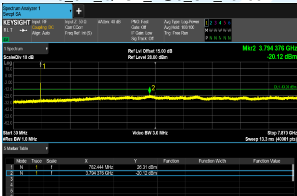
B13_5M_QPSK_1@0_CH_23255
