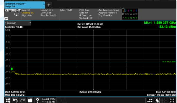
B13_5M_16QAM_1@0_CH_23205
