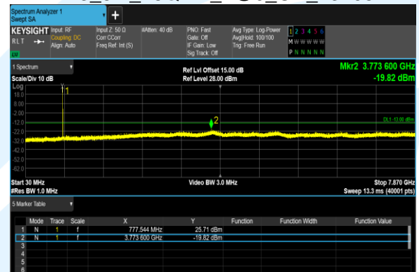
B13_5M_16QAM_1@0_CH_23205
