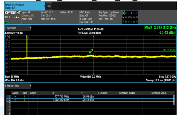
B13_10M_16QAM_1@0_CH_23230
