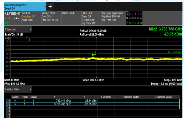
B13_5M_16QAM_1@0_CH_23255
