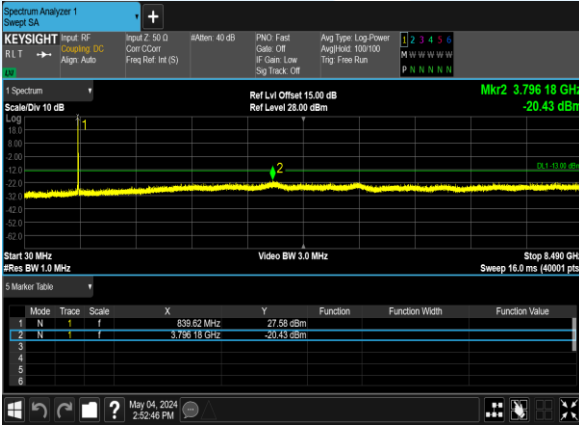
B5_5M_QPSK_1@0_CH_20425
