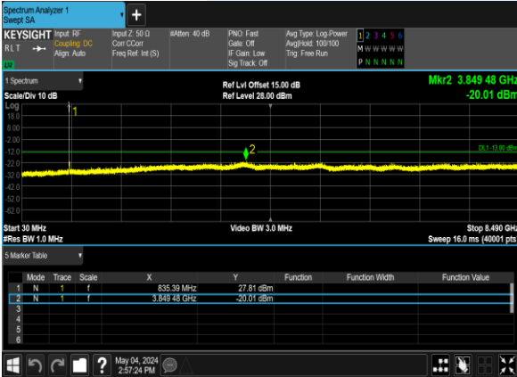
B5_3M_QPSK_1@0_CH_20525
