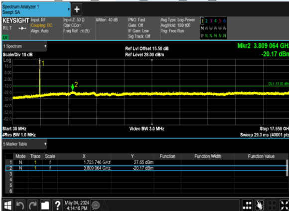
B4_20M_QPSK_1@0_CH_20175
