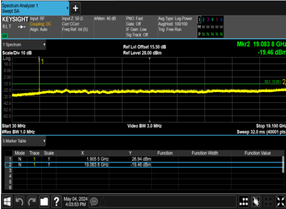
B2_5M_QPSK_1@0_CH_19175
