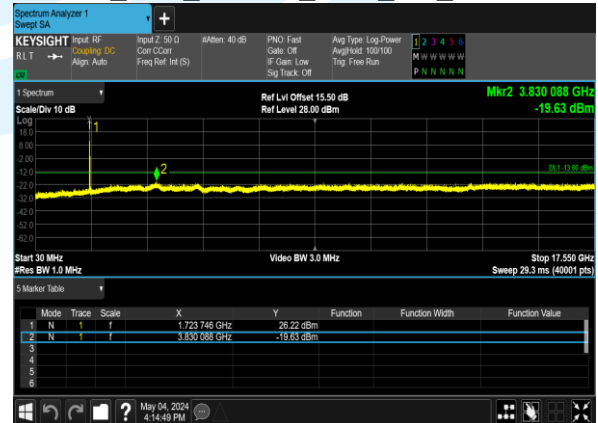
B4_20M_16QAM_1@0_CH_20175
