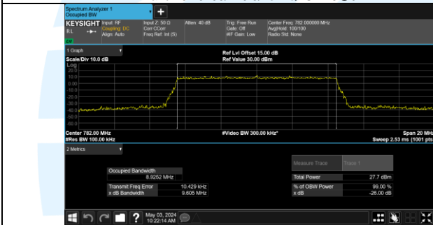
Band 13 23230/782.0/Low QPSK 50@0
