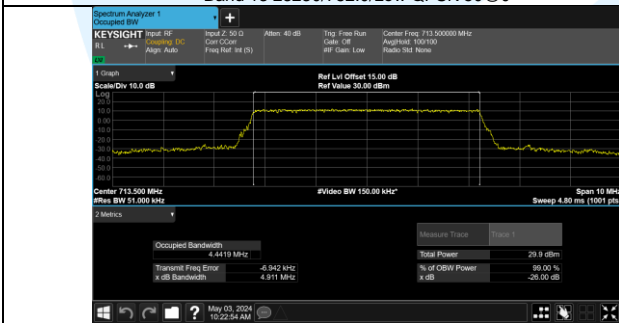
Band 17 23825/713.5/High QPSK 25@0
