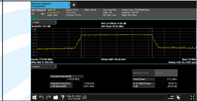
Band 13 23205/779.5/Low 16QAM 25@0
