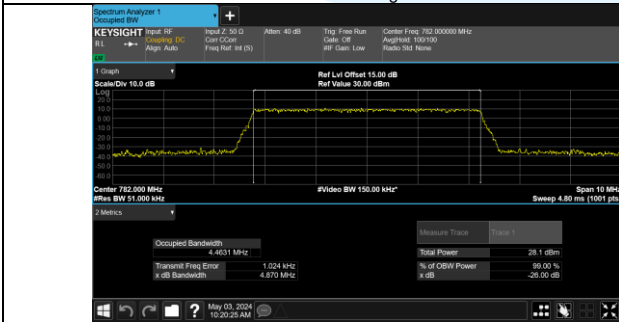
Band 13 23230/782.0/Mid QPSK 25@0
