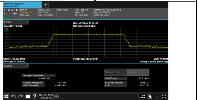
Band 13 23230/782.0/Mid 16QAM 25@0
