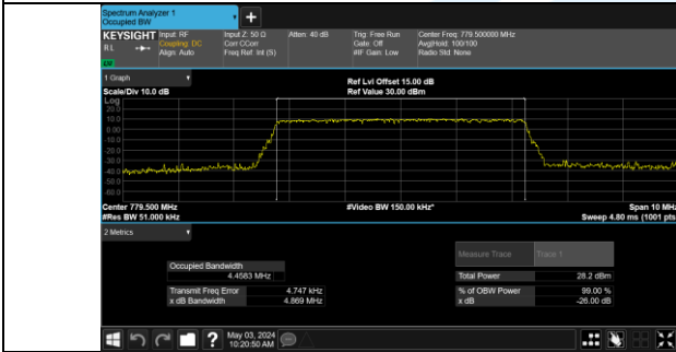
Band 13 23205/779.5/Low QPSK 25@0
