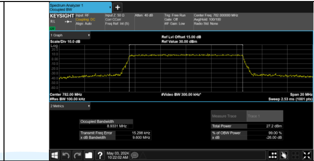
Band 13 23230/782.0/Mid 16QAM 50@0
