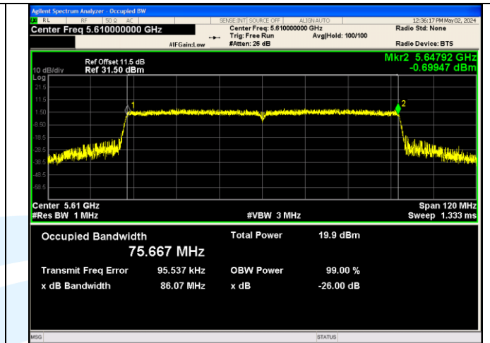
IEEE 802.11ac_Channel 122_80MHz_Antenna 0
