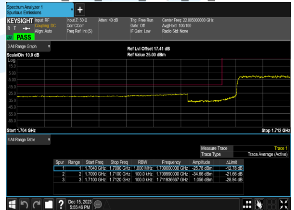
B4_10M_QPSK_50@0_CH_20000
