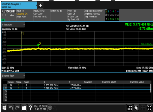
B4_1.4M_QPSK_1@0_CH_20393
