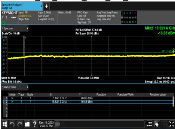
B2_5M_QPSK_1@0_CH_18900
