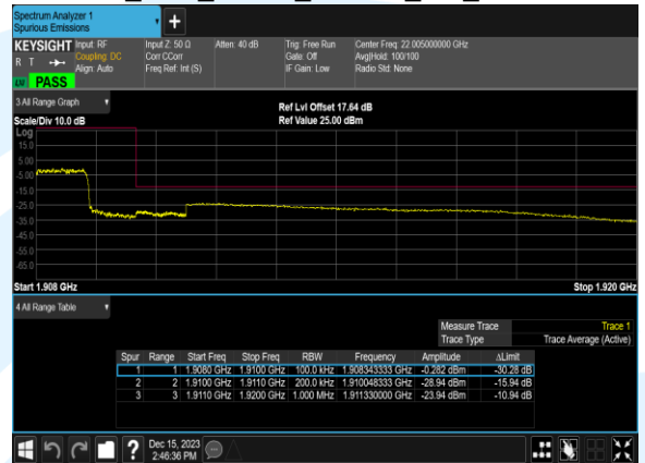
B2_20M_16QAM_100@0_CH_19100
