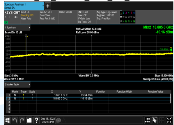
B2_5M_16QAM_1@0_CH_18900
