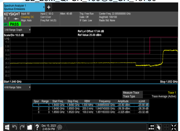
B2_20M_QPSK_100@0_CH_18700
