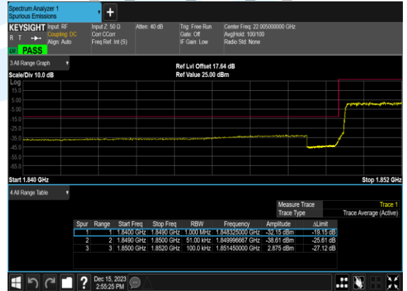
B2_5M_QPSK_25@0_CH_18625
