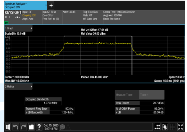
B2_1.4M_16QAM_6@0_CH_19193
