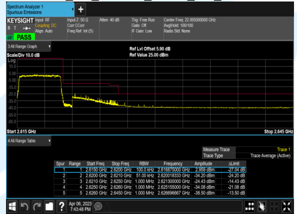
B38_20M_64QAM_100@0_CH_37850
