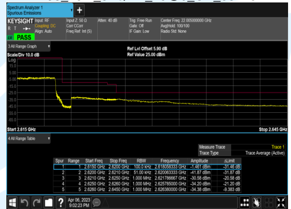
B38_10M_64QAM_50@0_CH_37800
