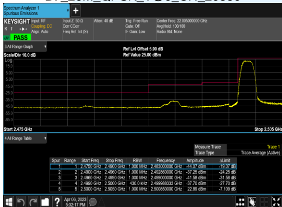
B7_20M_QPSK_1@0_CH_20850
