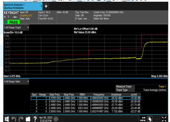
B7_20M_QPSK_100@0_CH_20850
