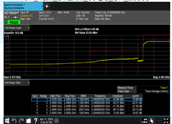
B7_10M_64QAM_50@0_CH_20800
