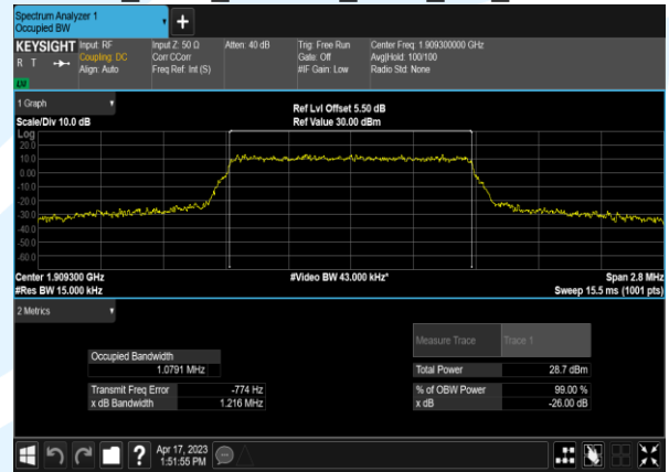
B2_1.4M_16QAM_6@0_CH_19193
