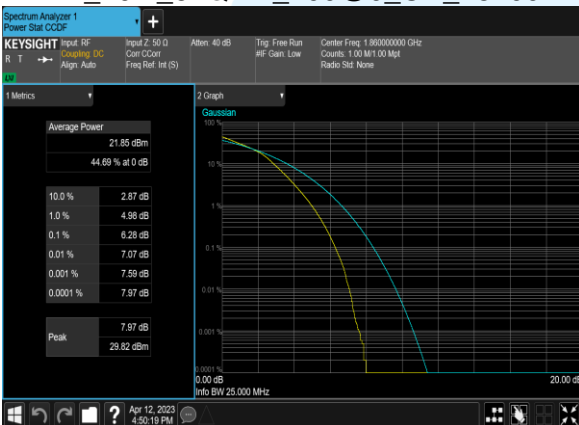
B2_20M_64QAM_100@0_CH_18700
