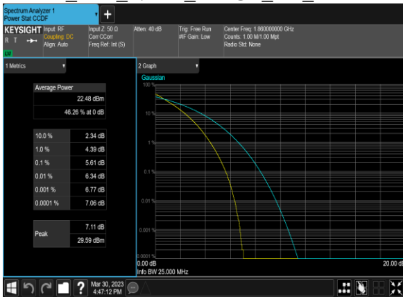
B2_20M_QPSK_100@0_CH_18900
