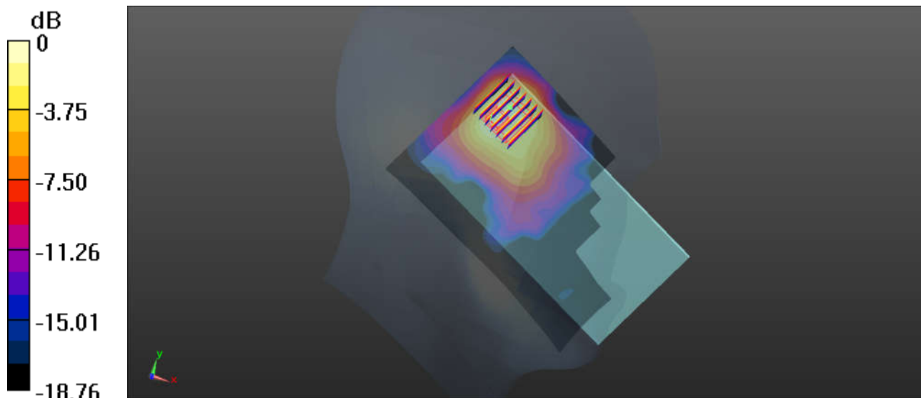
0 dB = 0.867 W/kg
