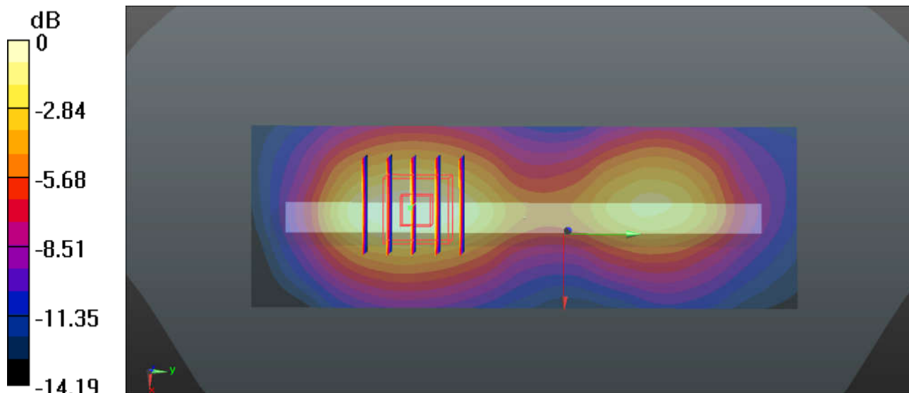
0 dB = 0.120 W/kg
