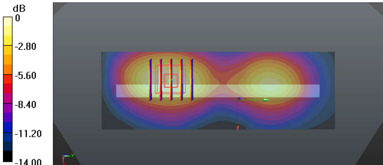
0 dB = 0.130 W/kg
