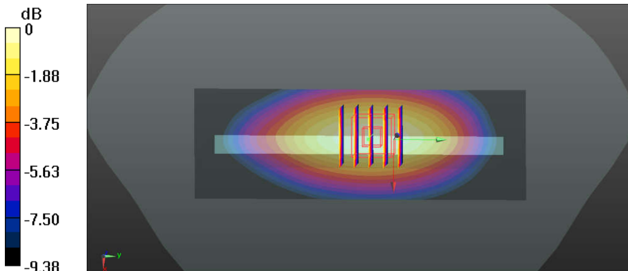
0 dB = 0.272 W/kg
