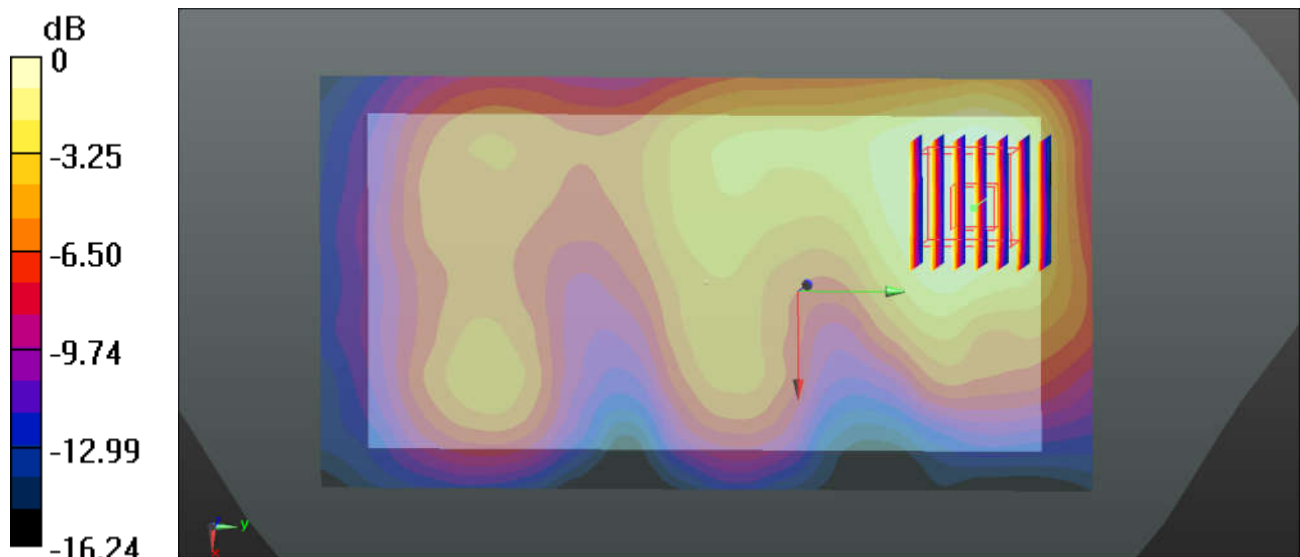
0 dB = 0.161 W/kg
