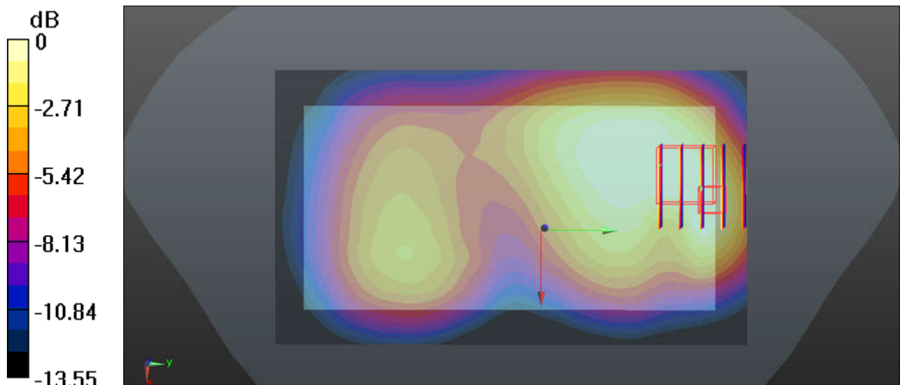
0 dB = 0.177 W/kg
