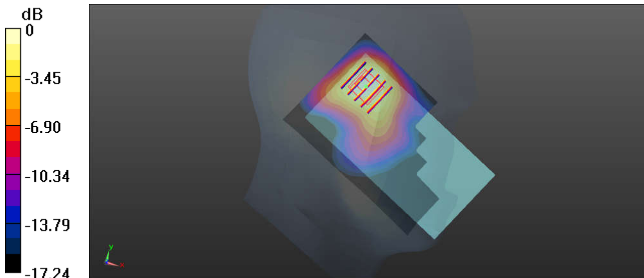
0 dB = 0.537 W/kg
