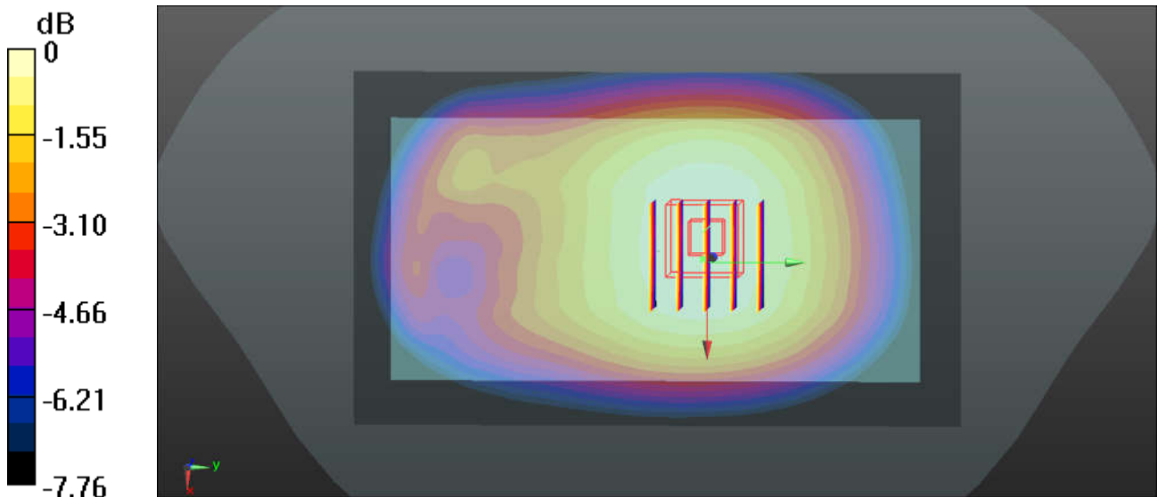
0 dB = 0.557 W/kg
