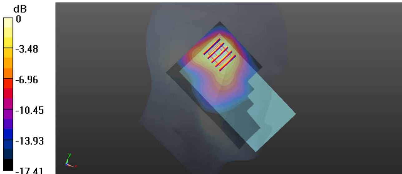
0 dB = 0.605 W/kg
