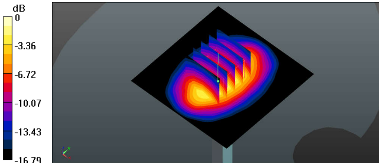
0 dB = 13.9 W/kg
