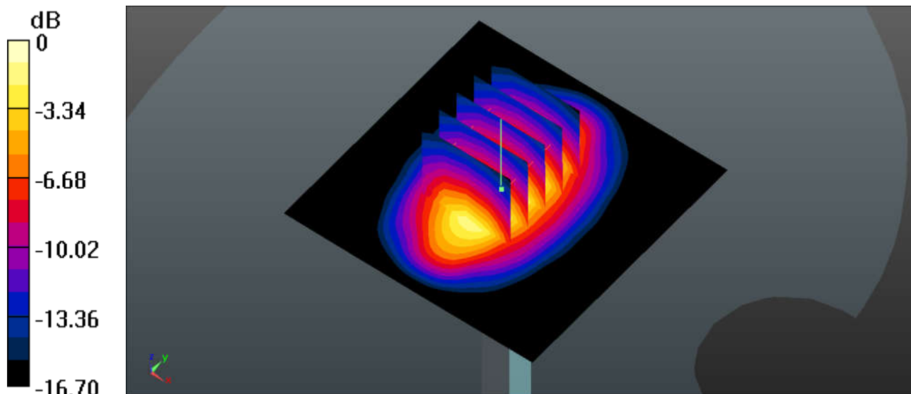
0 dB = 13.3 W/kg
