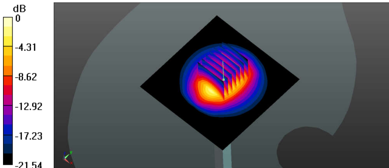
0 dB = 19.7 W/kg
