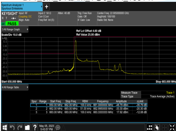
B71_5M_64QAM_1@0_CH_133147
