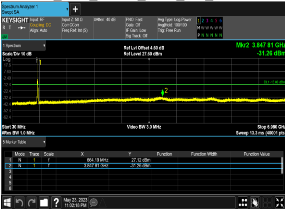
B71_20M_QPSK_1@0_CH_133322
