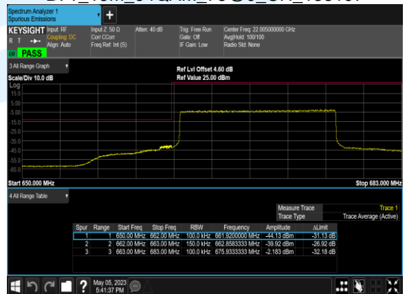
B71_15M_64QAM_75@0_CH_133197
