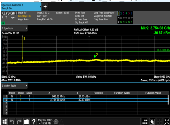
B71_5M_QPSK_1@0_CH_133147
