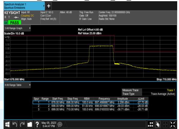
B71_5M_64QAM_25@0_CH_133447
