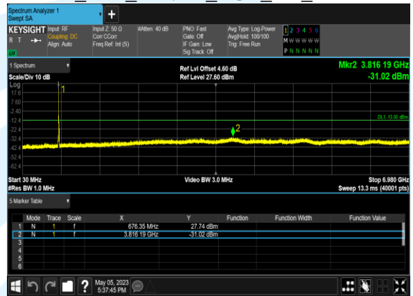
B71_5M_64QAM_1@0_CH_133147
