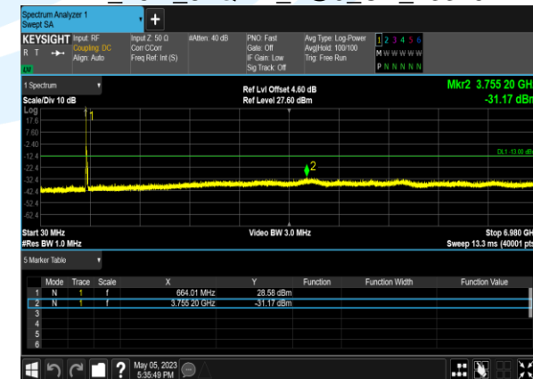
B71_15M_64QAM_1@0_CH_133197
