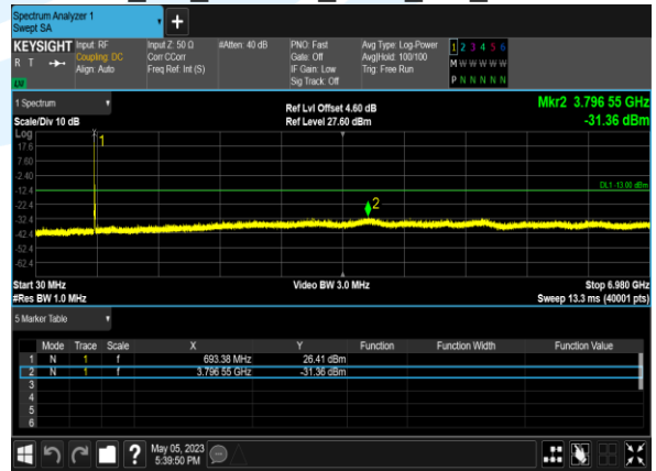
B71_5M_64QAM_1@0_CH_133447
