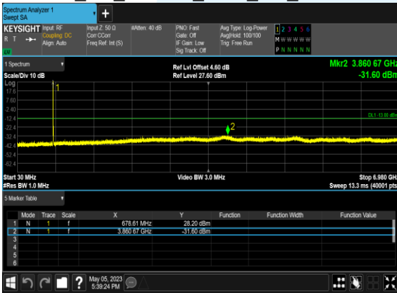
B71_5M_64QAM_1@0_CH_133297
