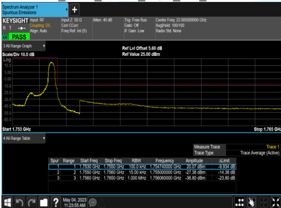
B4_1.4M_QPSK_1@5_CH_20393
