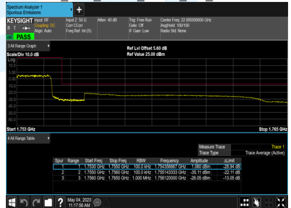
B4_10M_QPSK_50@0_CH_20350
