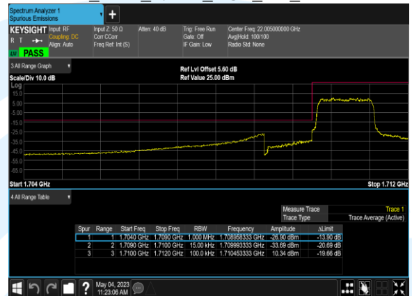
B4_1.4M_16QAM_6@0_CH_19957
