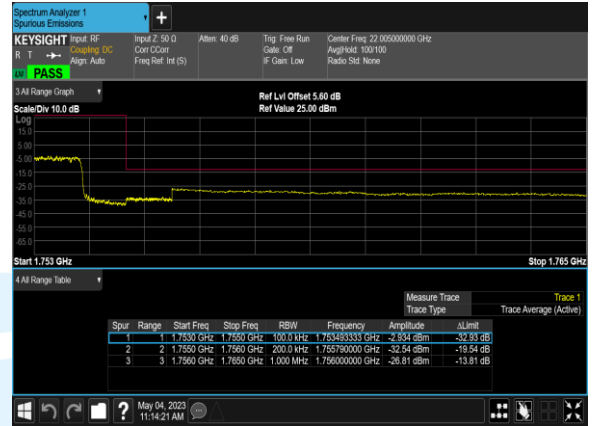
B4_15M_QPSK_75@0_CH_2025
