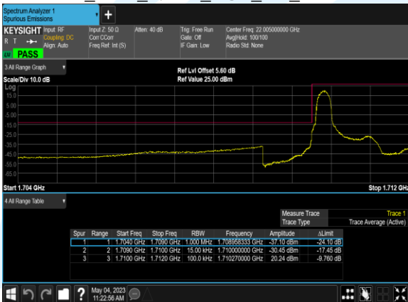
B4_1.4M_16QAM_1@0_CH_19957
