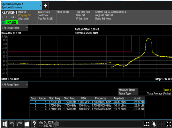
B4_15M_16QAM_1@0_CH_2025
