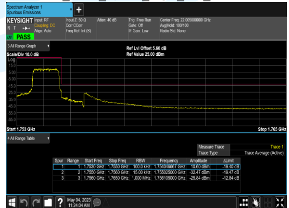
B4_1.4M_QPSK_6@0_CH_20393
