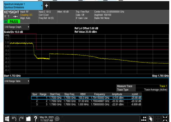
B4_5M_QPSK_25@0_CH_20375
