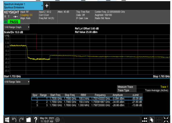
B4_15M_QPSK_75@0_CH_20325
