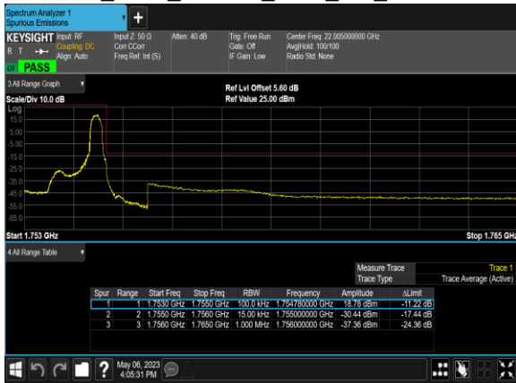
B4_1.4M_64QAM_1@5_CH_20393
