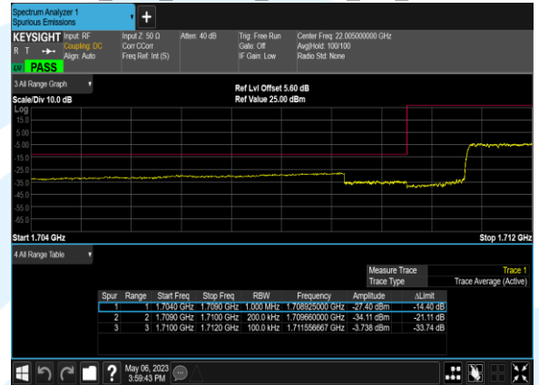
B4_20M_64QAM_100@0_CH_20300
