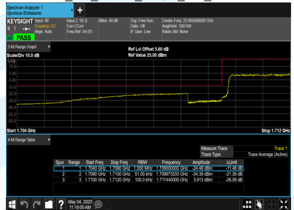
B4_5M_16QAM_25@0_CH_19975
