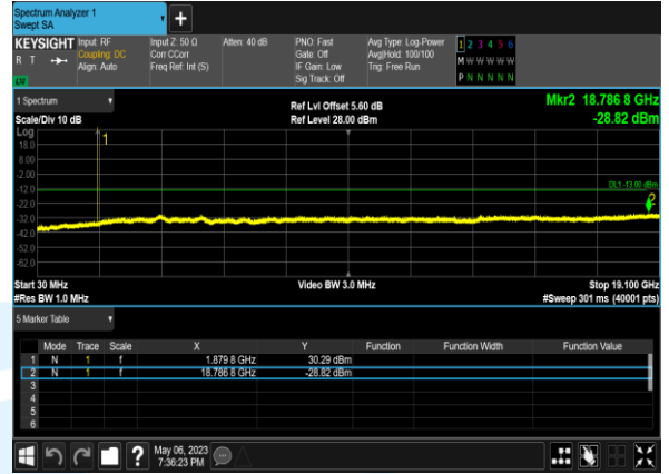
EGPRS1900_Channel661
