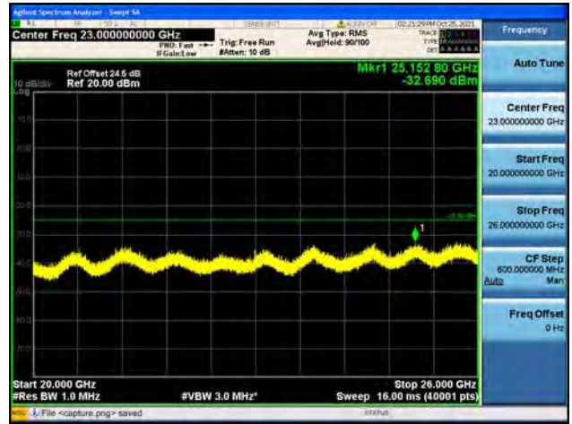
Band7 / 20MHz / Mid CH / 16QAM
