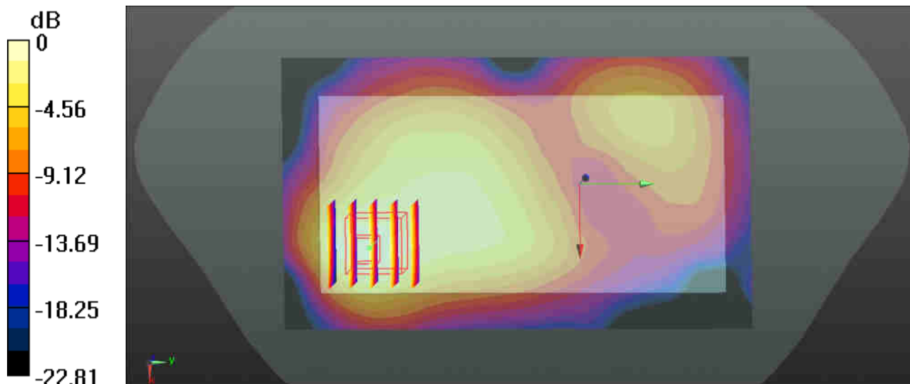
0 dB = 0.193 W/kg
