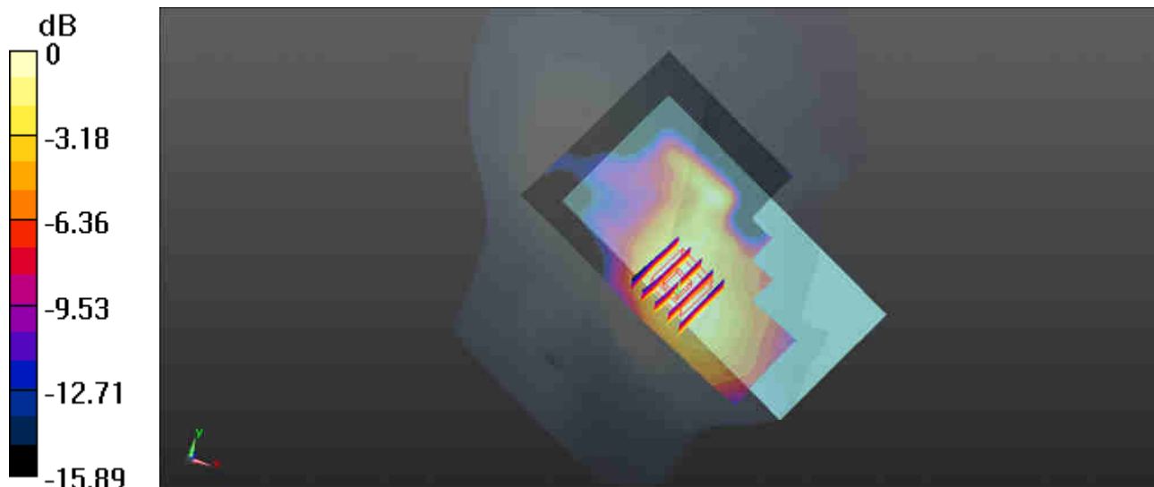
0 dB = 0.0881 W/kg
