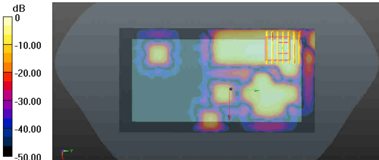
0 dB = 0.0192 W/kg
