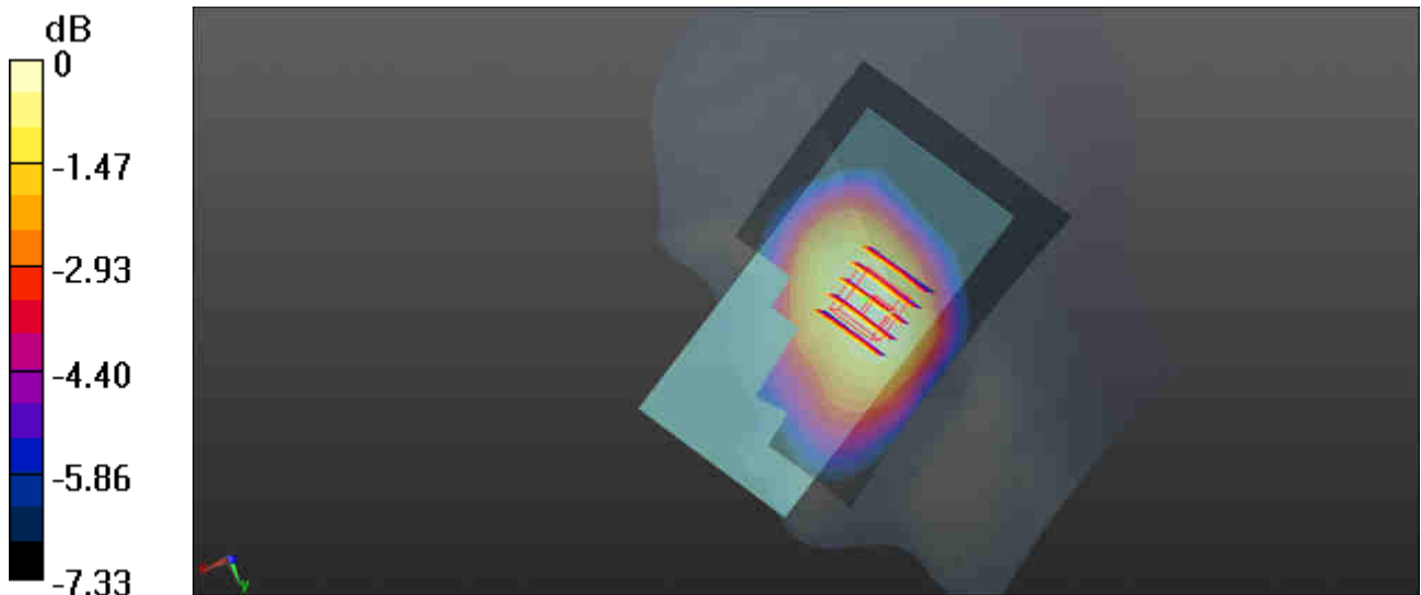
0 dB = 0.176 W/kg
