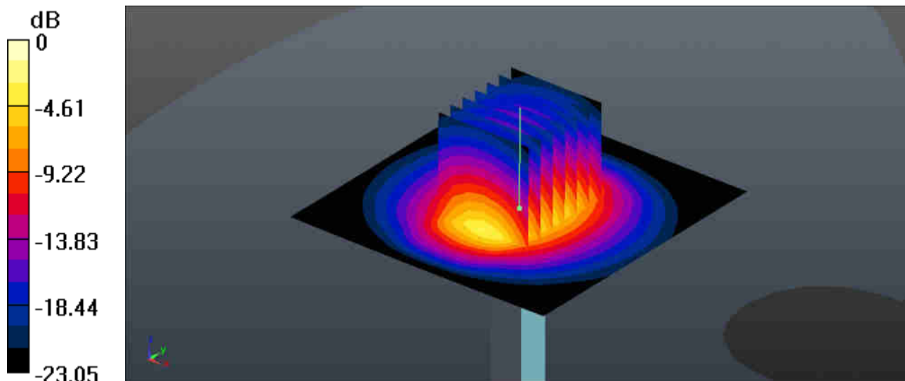
0 dB = 22.6 W/kg
