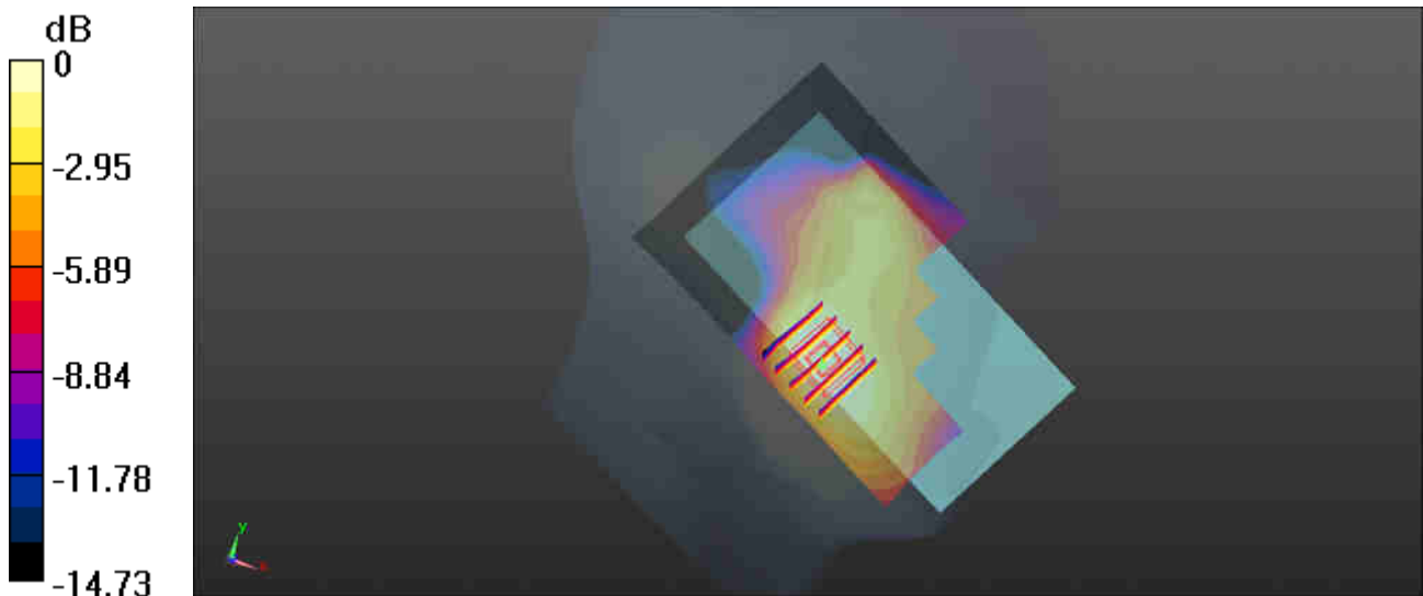
0 dB = 0.0681 W/kg
