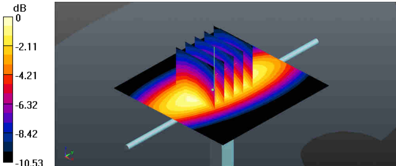
0 dB = 3.12 W/kg
