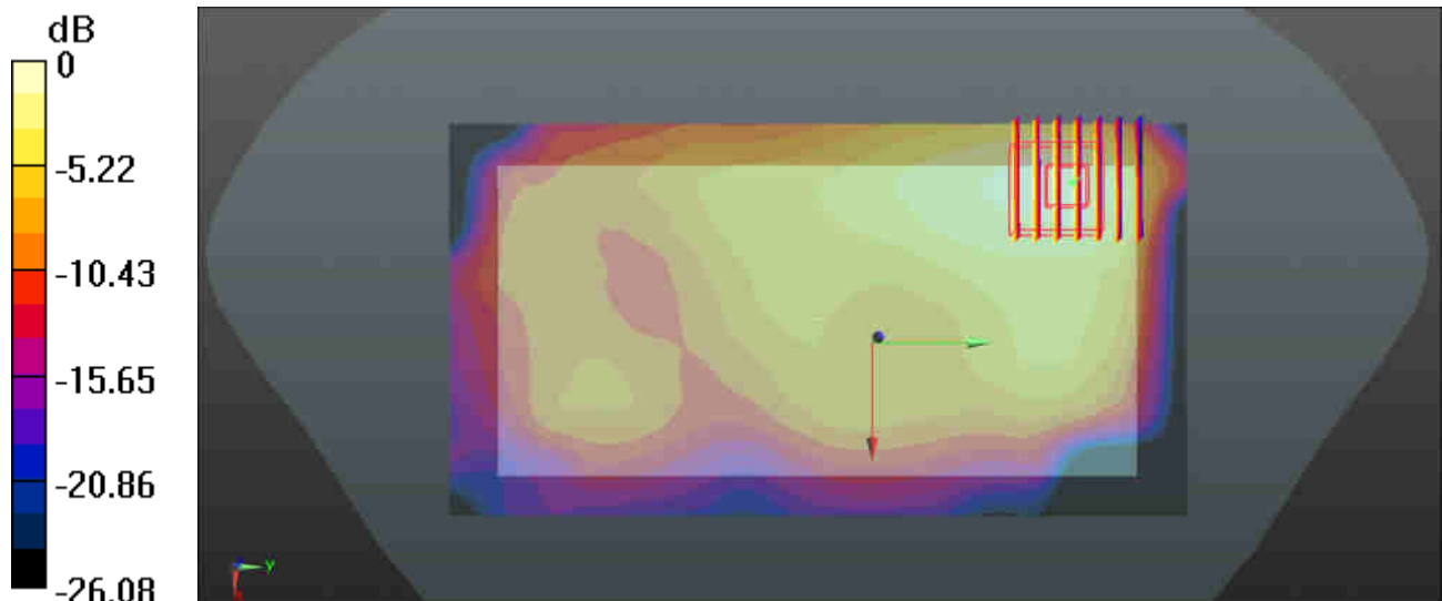
0 dB = 0.215 W/kg
