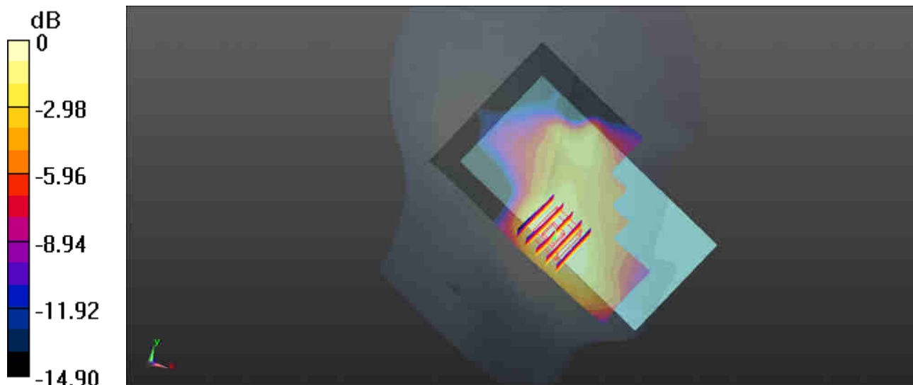
0 dB = 0.0651 W/kg
