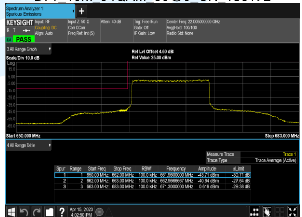
B71_10M_64QAM_50@0_CH_133172
