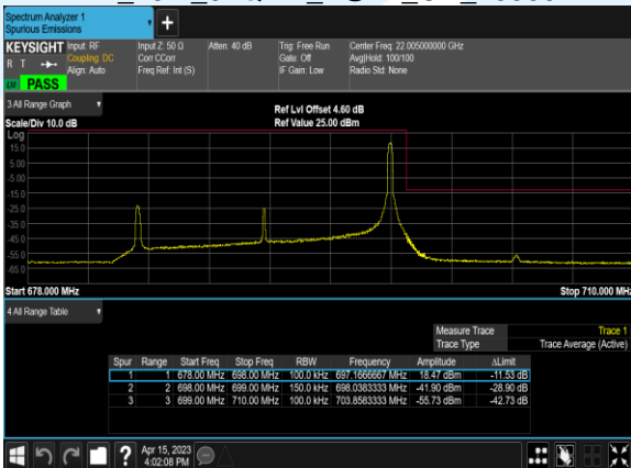
B71_10M_64QAM_1@0_CH_133172
