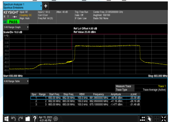
B71_15M_64QAM_75@0_CH_133397
