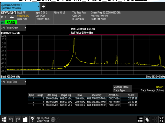
B71_20M_64QAM_1@0_CH_133222
