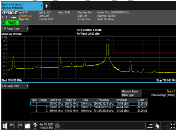
B71_15M_64QAM_1@0_CH_133197
