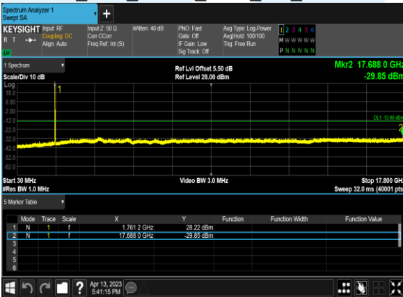
B66_20M_QPSK_1@0_CH_132572
