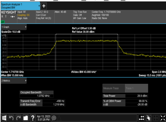
B66_1.4M_QPSK_6@0_CH_132322
