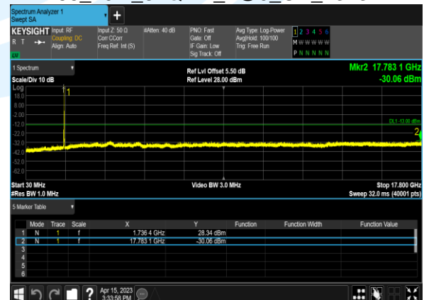
B66_20M_64QAM_1@0_CH_132322
