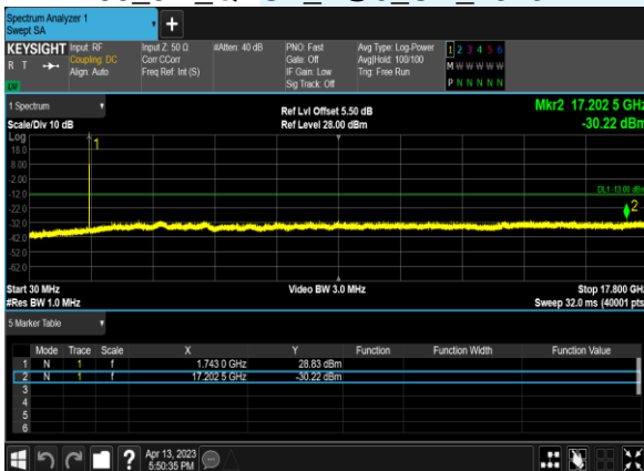
B66_5M_QPSK_1@0_CH_132322
