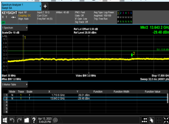
B66_5M_QPSK_1@0_CH_132322
