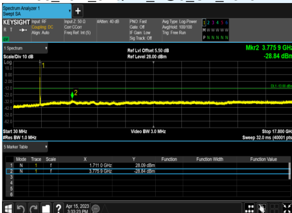
B66_20M_64QAM_1@0_CH_132072
