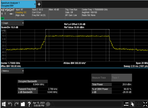
B4_10M_64QAM_50@0_CH_20350
