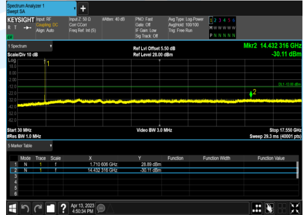
B4_10M_16QAM_1@0_CH_20000
