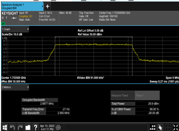
B4_3M_QPSK_15@0_CH_20385
