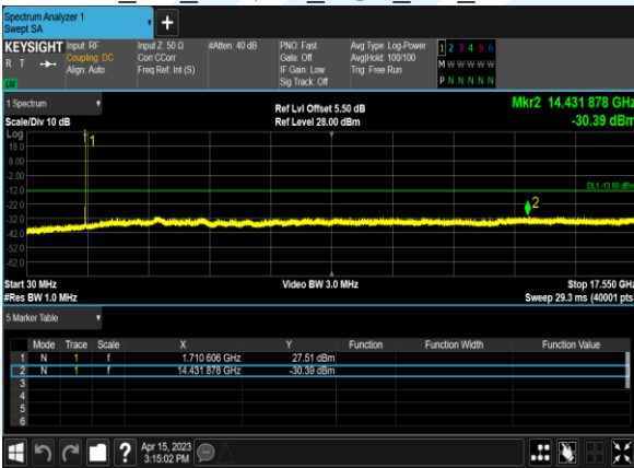
B4_3M_64QAM_1@0_CH_20385
