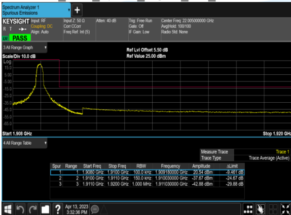
B2_15M_QPSK_1@74_CH_19125
