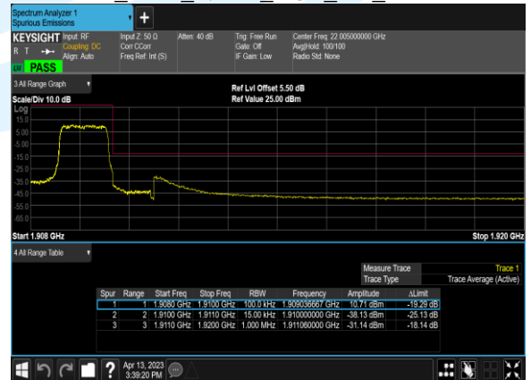
B2_1.4M_QPSK_6@0_CH_19193
