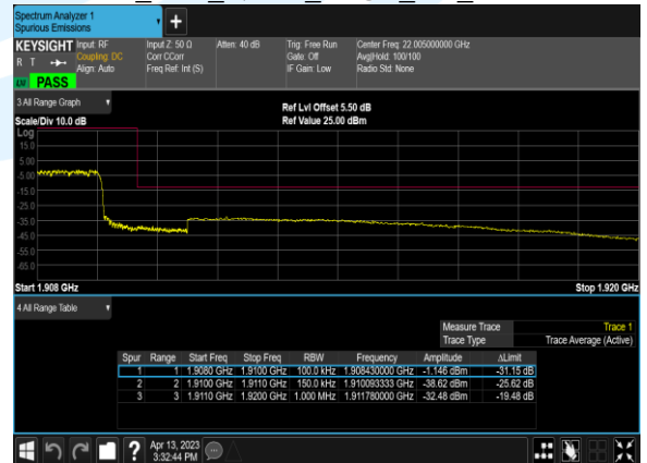
B2_15M_QPSK_75@0_CH_19125
