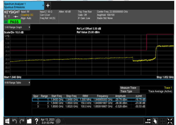
B2_15M_16QAM_75@0_CH_18675
