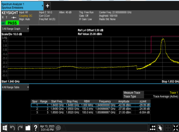
B2_15M_16QAM_1@0_CH_18675
