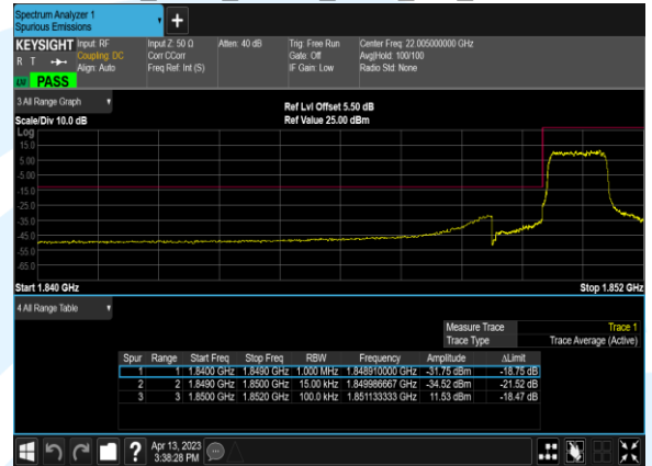
B2_1.4M_16QAM_6@0_CH_18607
