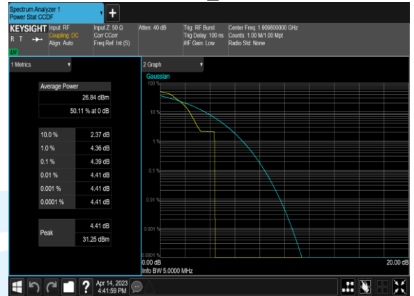
EGPRS1900_Channel810
