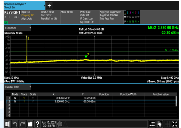
EGPRS850_Channel190
