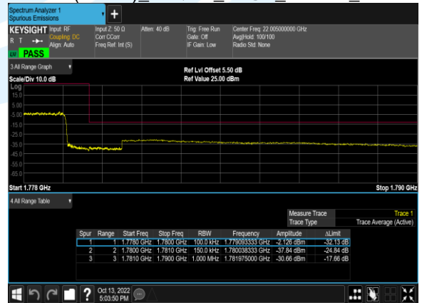
B66(15.0M)_64QAM_75@0_132597_CH
