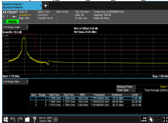
B66(15.0M)_64QAM_1@74_132597_CH
