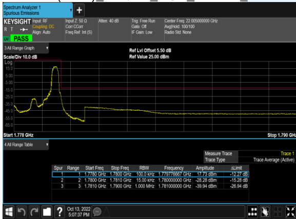
B66(1.4M)_64QAM_1@5_132665_CH
