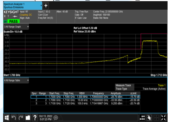
B66(1.4M)_64QAM_6@0_132665_CH
