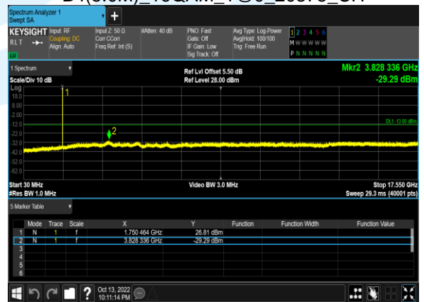
B4(5.0M)_16QAM_1@0_20375_CH
