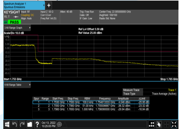
B4(5.0M)_16QAM_25@0_20375_CH
