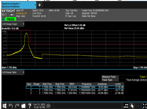
B4(5.0M)_16QAM_1@24_20375_CH
