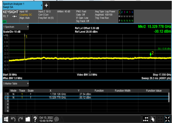
B4(5.0M)_64QAM_1@0_19975_CH
