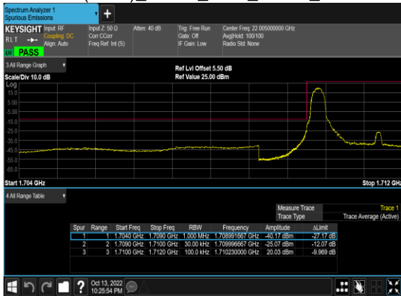
B4(3.0M)_16QAM_1@0_19965_CH
