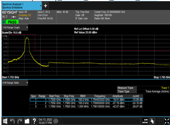
B4(10.0M)_16QAM_1@49_20350_CH
