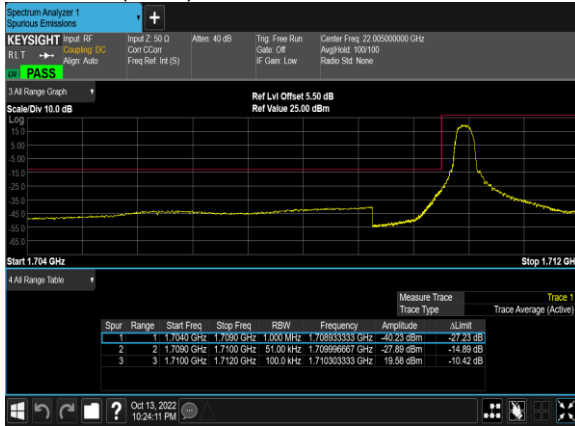
B4(5.0M)_16QAM_1@0_19975_CH
