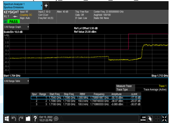
B4(15.0M)_16QAM_75@0_20025_CH
