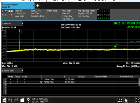
B4(1.4M)_QPSK_1@0_19957_CH
