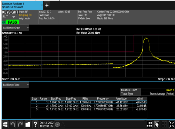
B4(10.0M)_16QAM_1@0_20000_CH
