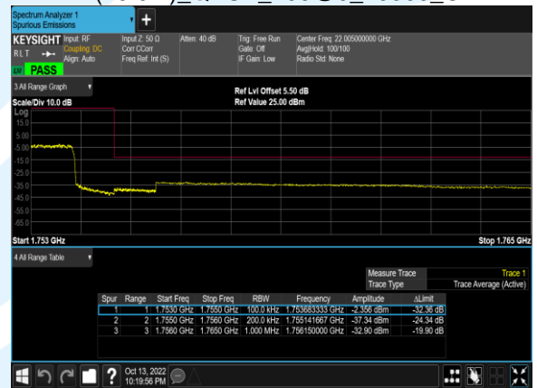
B4(20.0M)_16QAM_100@0_20300_CH
