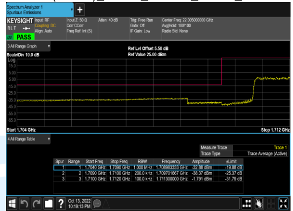
B4(20.0M)_16QAM_100@0_20050_CH
