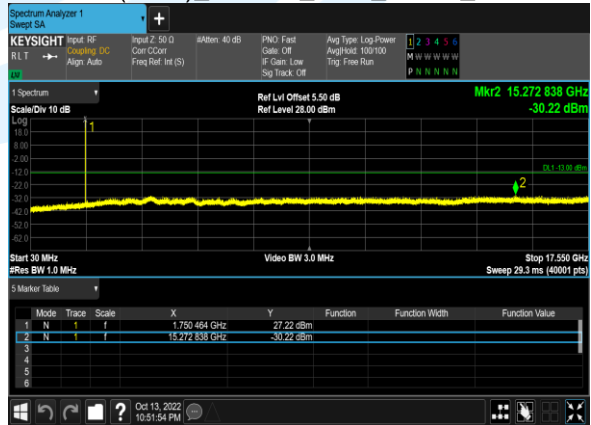
B4(5.0M)_64QAM_1@0_20375_CH
