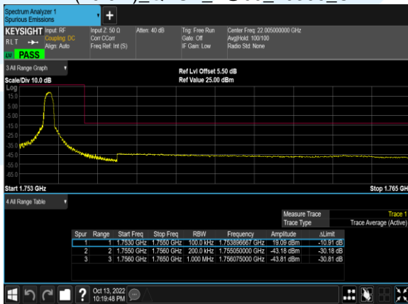
B4(20.0M)_16QAM_1@99_20300_CH
