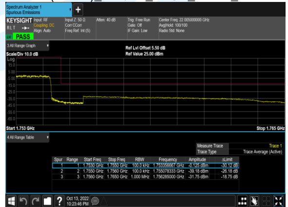
B4(10.0M)_16QAM_50@0_20350_CH
