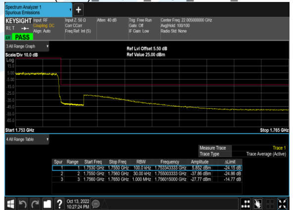
B4(3.0M)_16QAM_15@0_20385_CH
