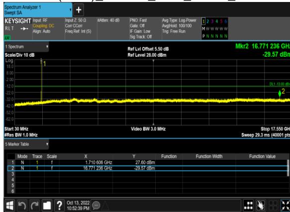
B4(3.0M)_64QAM_1@0_20385_CH
