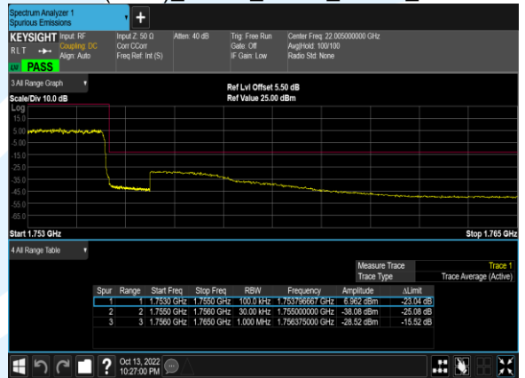
B4(3.0M)_16QAM_15@0_20385_CH
