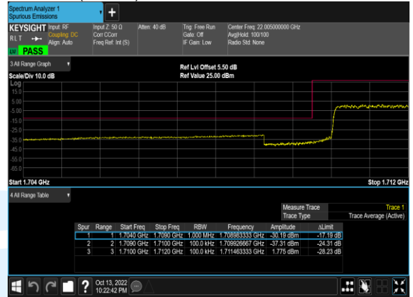
B4(10.0M)_16QAM_50@0_20000_CH
