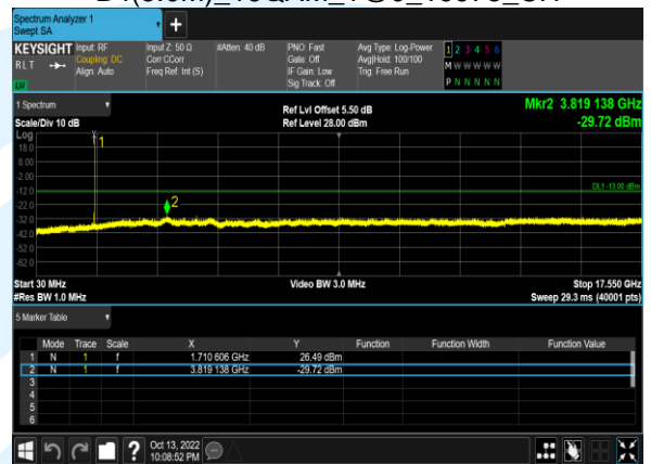
B4(5.0M)_16QAM_1@0_20175_CH
