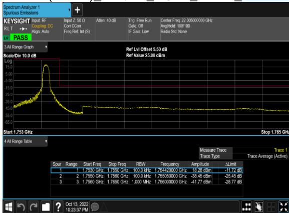
B4(10.0M)_16QAM_1@49_20350_CH
