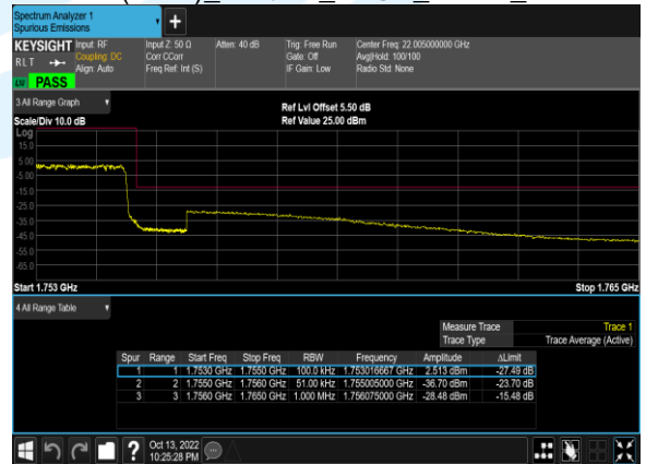
B4(5.0M)_16QAM_25@0_20375_CH
