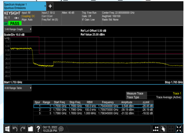
B4(10.0M)_16QAM_50@0_20350_CH
