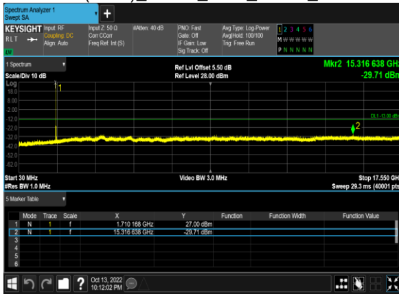
B4(3.0M)_QPSK_1@0_20175_CH
