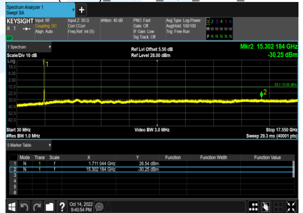
B4(15.0M)_64QAM_1@0_2025_CH
