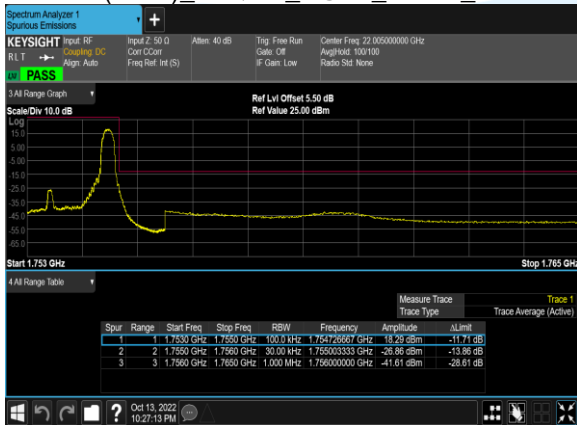
B4(3.0M)_16QAM_1@14_20385_CH
