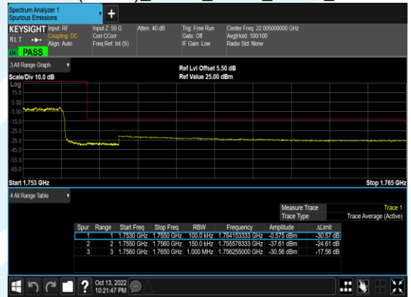
B4(15.0M)_16QAM_75@0_20325_CH
