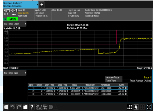
B4(5.0M)_16QAM_25@0_19975_CH
