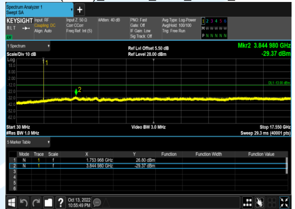
B4(1.4M)_64QAM_1@0_20393_CH
