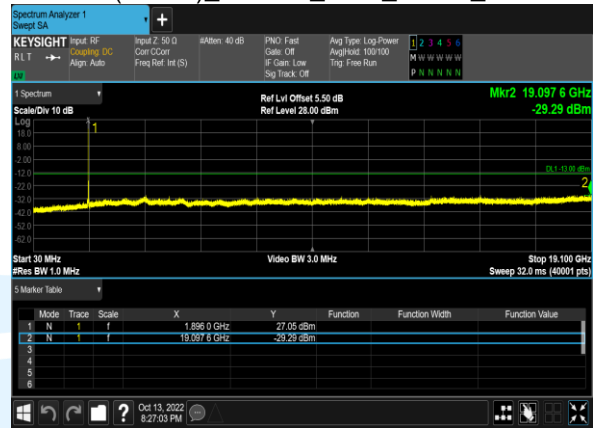
B2(10.0M)_64QAM_1@0_18900_CH
