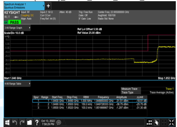
B2(15.0M)_16QAM_75@0_18675_CH
