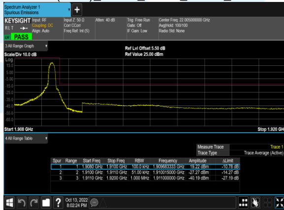
B2(5.0M)_16QAM_1@24_19175_CH
