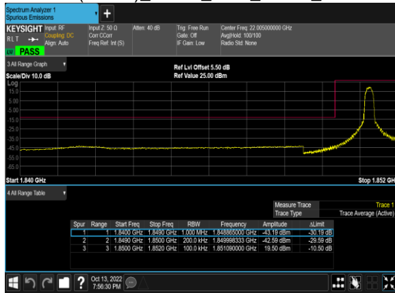
B2(20.0M)_16QAM_1@0_18700_CH
