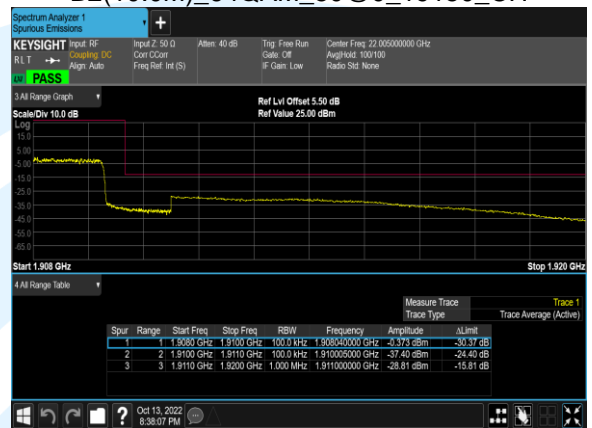
B2(5.0M)_64QAM_25@0_18625_CH
