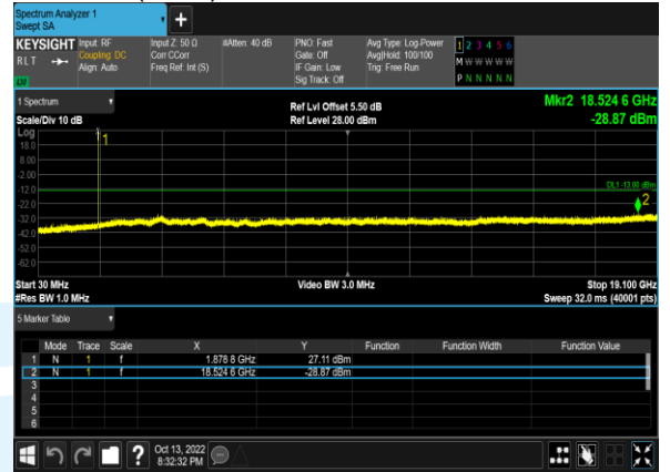
B2(1.4M)_64QAM_1@0_18607_CH
