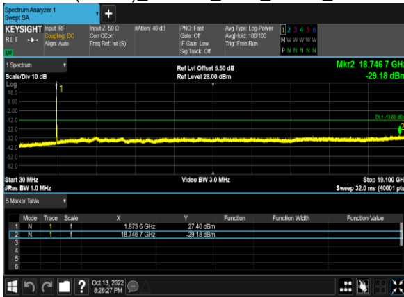
B2(10.0M)_64QAM_1@0_18650_CH
