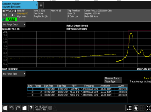
B2(1.4M)_16QAM_1@0_18607_CH
