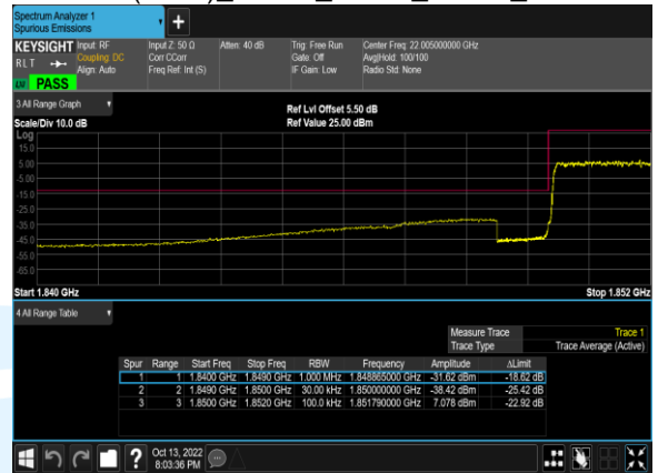
B2(3.0M)_16QAM_15@0_18615_CH
