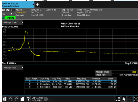
B2(3.0M)_16QAM_1@14_19185_CH
