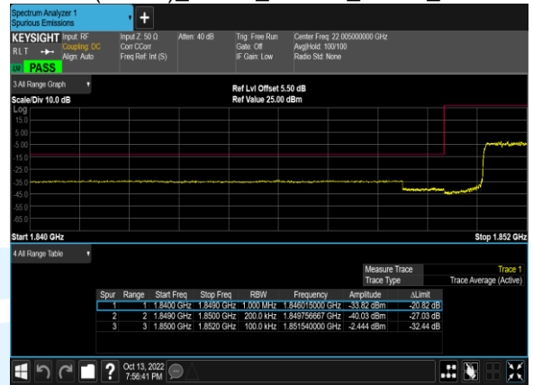
B2(20.0M)_16QAM_100@0_18700_CH
