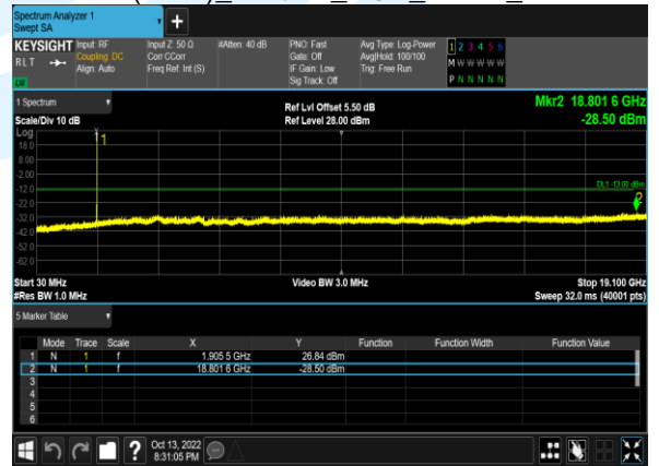
B2(5.0M)_64QAM_1@0_19175_CH
