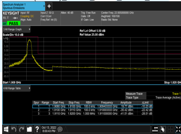
B2(10.0M)_16QAM_1@49_19150_CH
