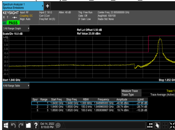
B2(15.0M)_16QAM_1@0_18675_CH
