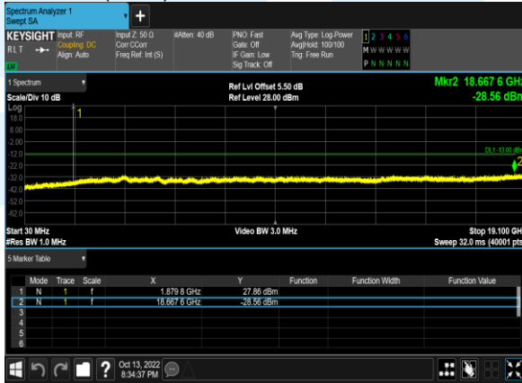
B2(1.4M)_64QAM_1@0_18900_CH
