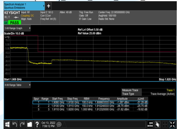
B2(15.0M)_16QAM_75@0_19125_CH
