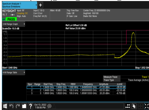
B2(10.0M)_16QAM_1@0_18650_CH
