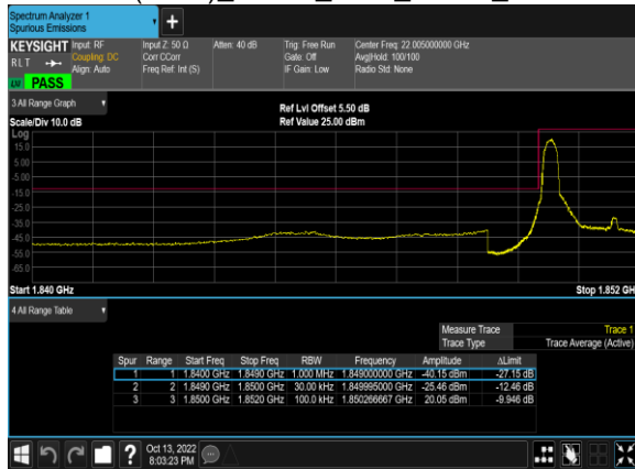
B2(3.0M)_16QAM_1@0_18615_CH
