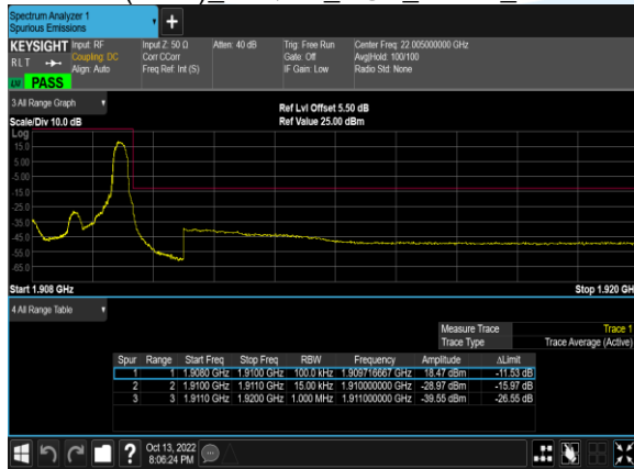
B2(1.4M)_16QAM_1@5_19193_CH
