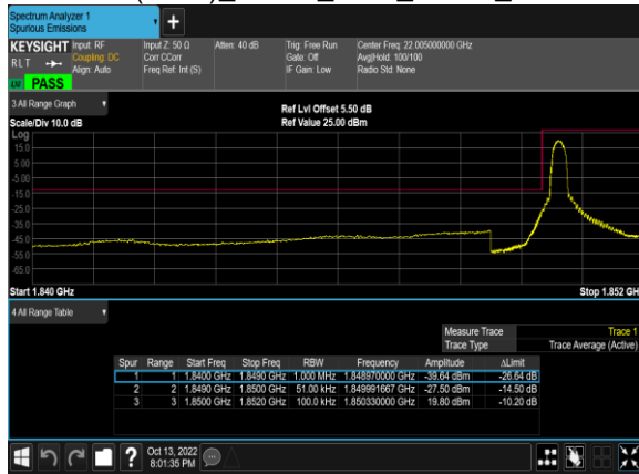
B2(5.0M)_16QAM_1@0_18625_CH
