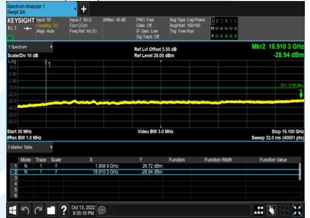
B2(1.4M)_64QAM_1@0_19193_CH
