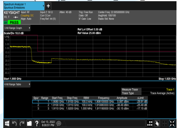
B2(10.0M)_16QAM_50@0_19150_CH
