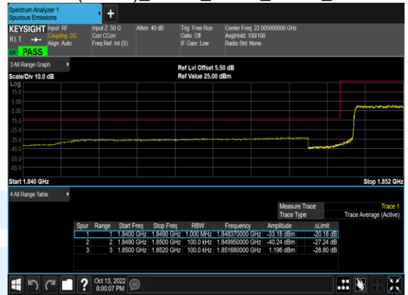
B2(10.0M)_16QAM_50@0_18650_CH
