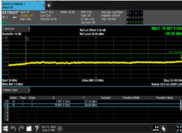
B2(1.4M)_64QAM_1@0_18900_CH
