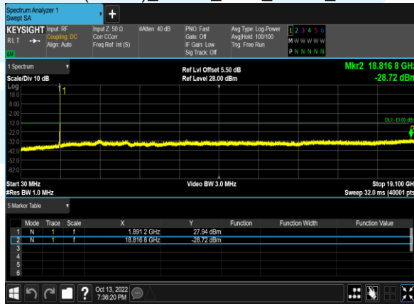
B2(15.0M)_QPSK_1@0_18675_CH
