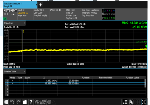
B2(1.4M)_16QAM_1@0_18607_CH
