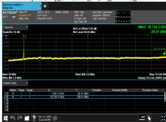
B2(20.0M)_64QAM_1@0_19100_CH
