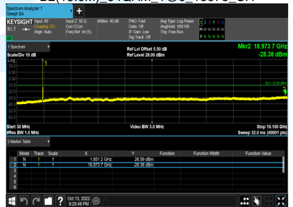
B2(15.0M)_64QAM_1@0_18675_CH
