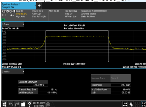
B2(5.0M)_64QAM_25@0_18900_CH
