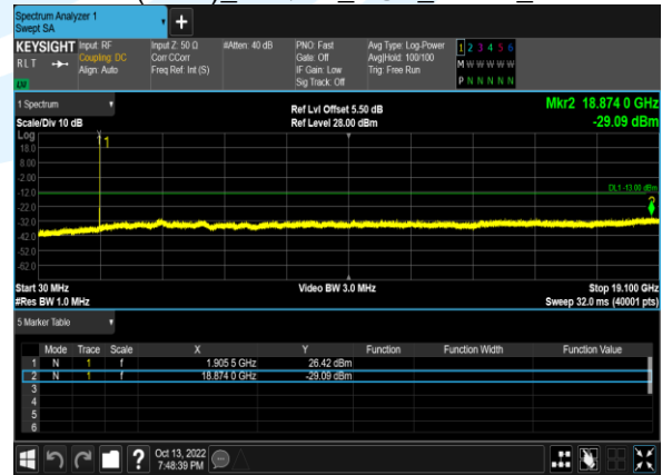
B2(5.0M)_16QAM_1@0_19175_CH
