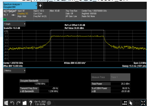
B2(1.4M)_16QAM_6@0_18607_CH
