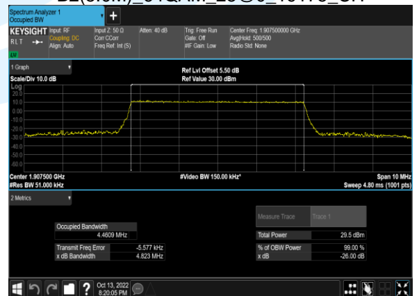
B2(5.0M)_64QAM_25@0_19175_CH
