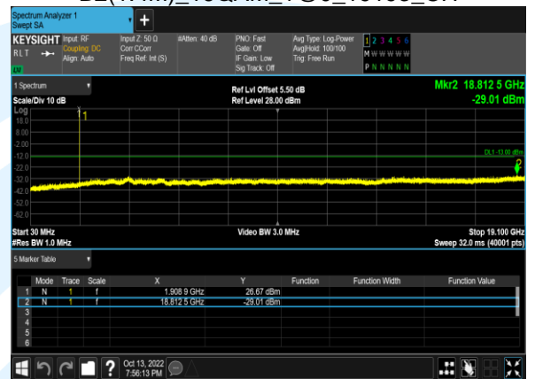
B2(20.0M)_64QAM_1@0_18900_CH
