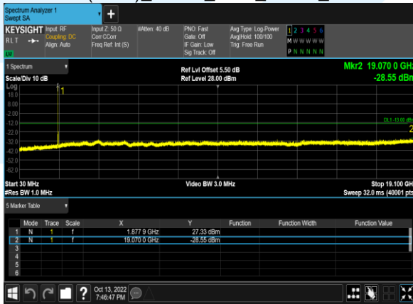
B2(5.0M)_QPSK_1@0_19175_CH
