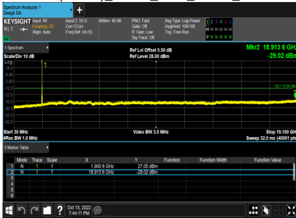
B2(5.0M)_QPSK_1@0_18625_CH
