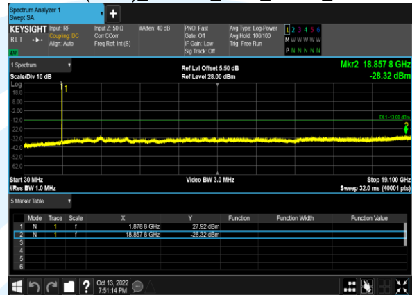
B2(3.0M)_16QAM_1@0_19185_CH
