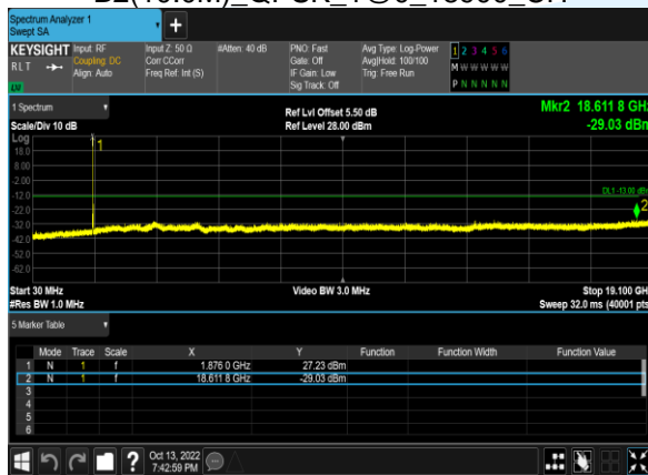
B2(10.0M)_QPSK_1@_18900_CH
