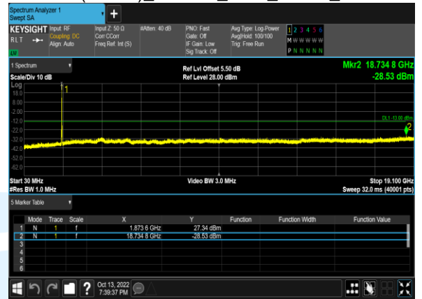
B2(15.0M)_16QAM_1@_19125_CH
