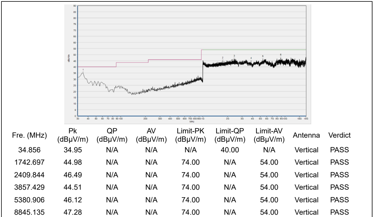
(Antenna Vertical, 30MHz to 18GHz)
